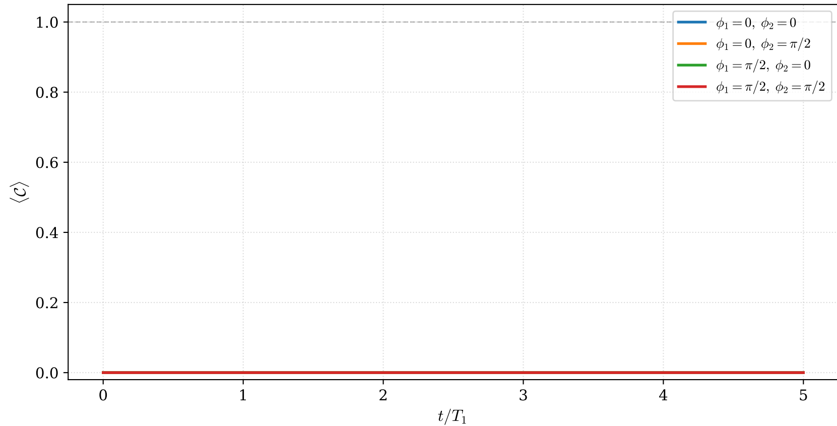
Ensemble-average concurrence -- PlusPlus, \eta_1 = 1.0 , \eta_2 = 0.0 , ntraj = 1000
