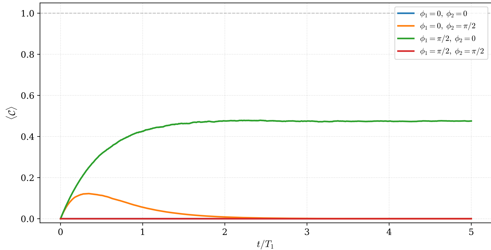
Ensemble-average concurrence -- PlusPlus, \eta_1 = 1.0 , \eta_2 = 0.5 , ntraj = 1000
