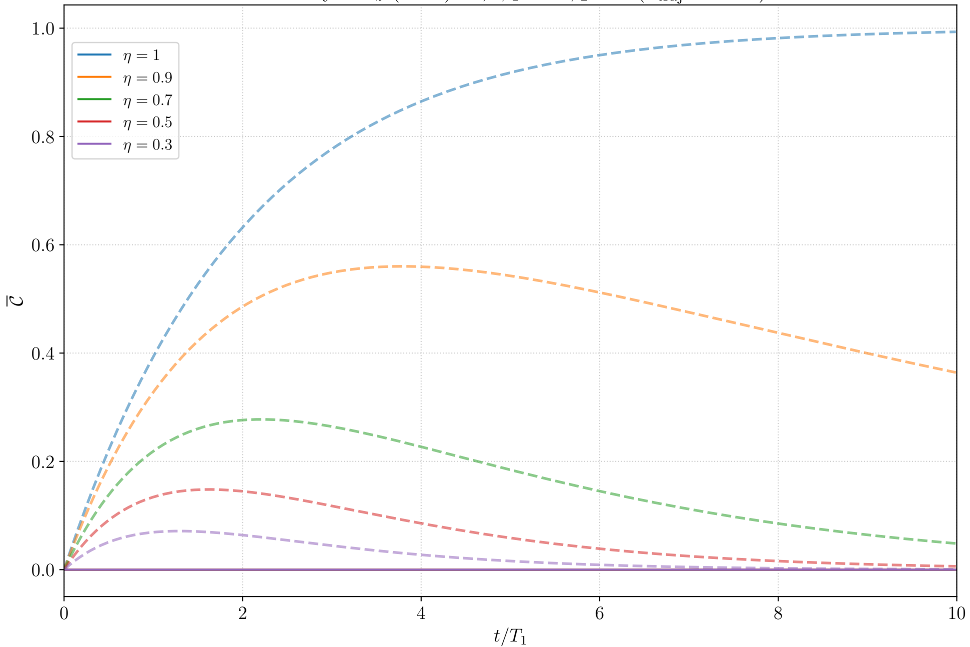
Homodyne J_z (N=2): \overline{\mathcal{C}} , \phi_1 = 0 \phi_2 = 0 ( n_{\text{traj}} = 1000 )
