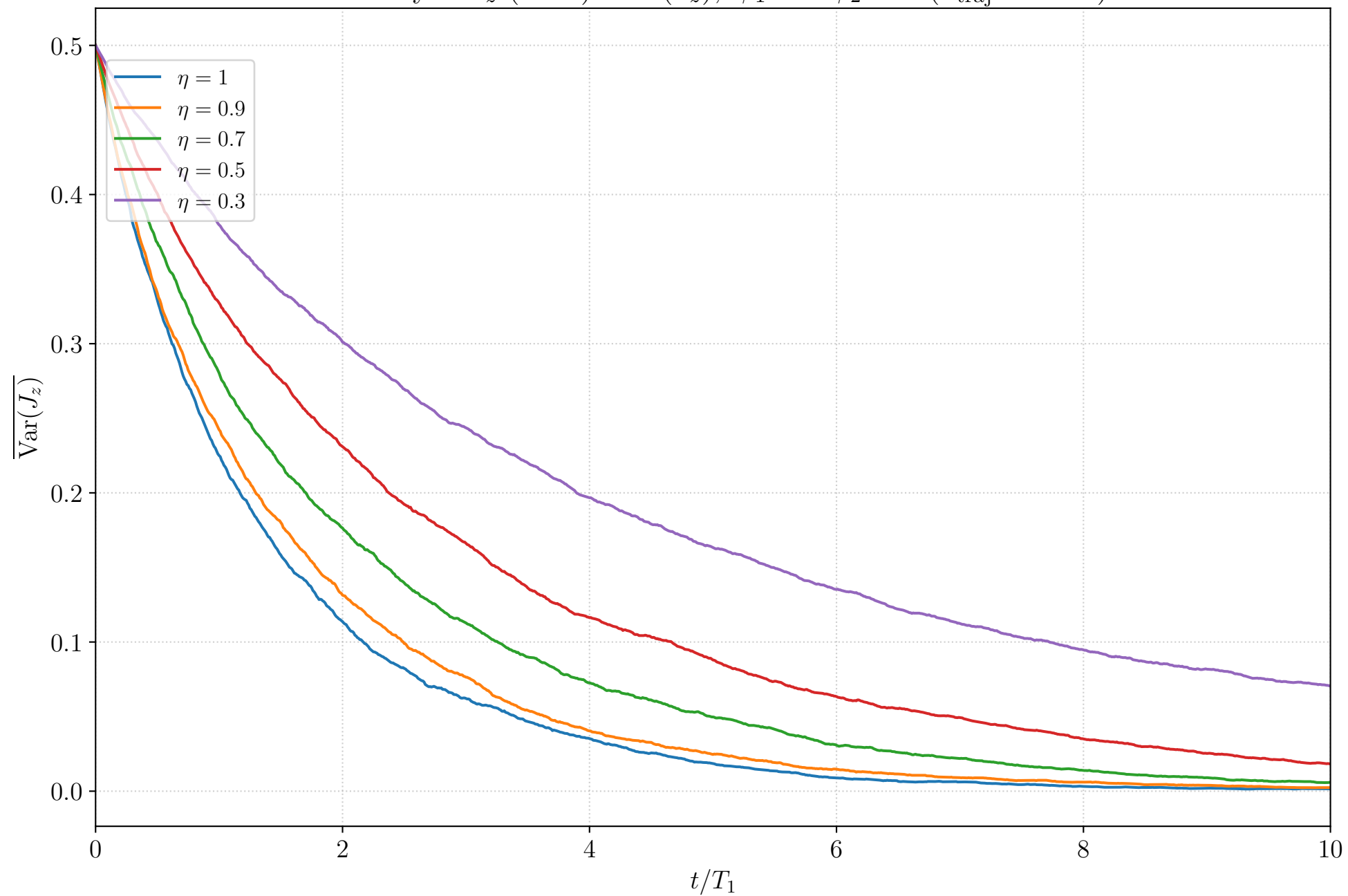
Homodyne J_z (N=2): \overline{\text{Var}(J_z)} , \phi_1 = 0 \phi_2 = 0 ( n_{\text{traj}} = 1000 )
