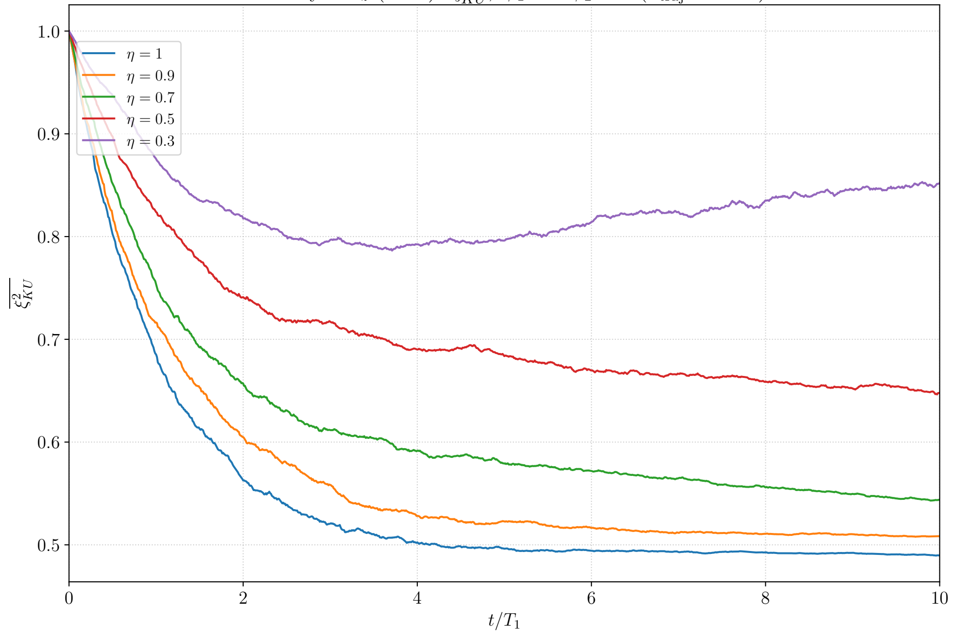
Homodyne J_z (N=2): \overline{\xi_{KU}^2} , \phi_1 = 0 \phi_2 = 0 ( n_{\text{traj}} = 1000 )
