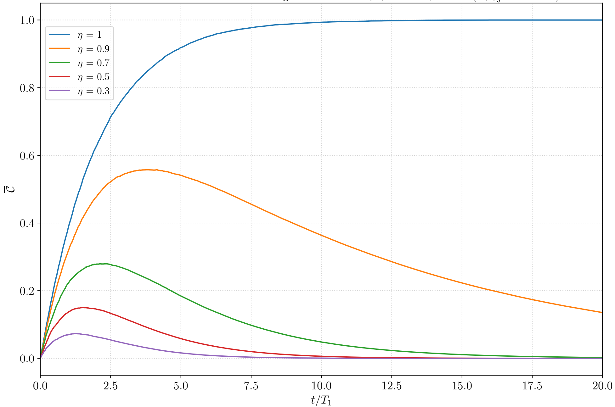
Inefficient Photodetection: Average \bar{\mathcal{C}} over time, \phi_1 = 0 \phi_2 = 0 ( n_{\text{traj}} = 10000 )
