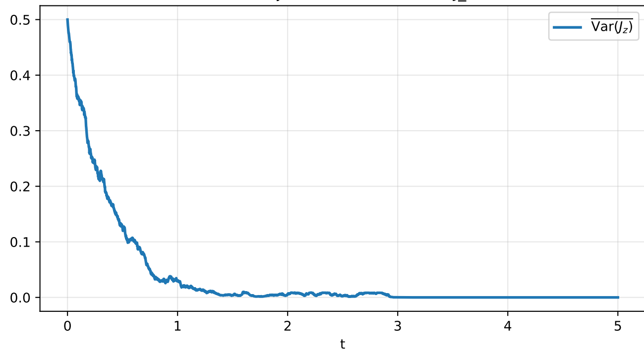
Ideal trajectories: Variance on J_z
