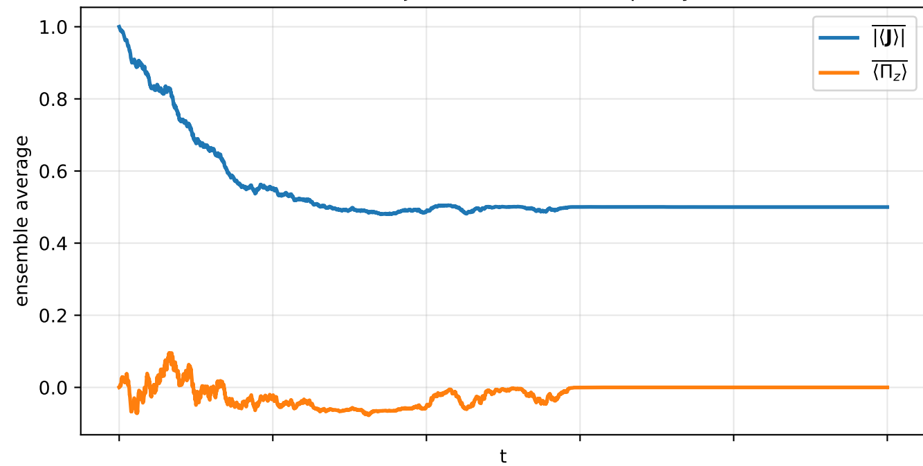
Ideal trajectories: Metrological gain
