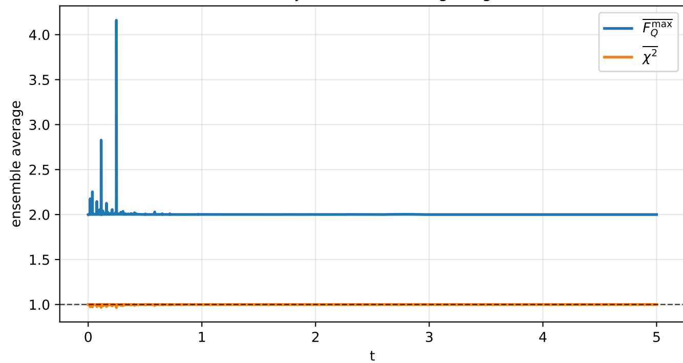
Ideal trajectories: Metrological gain
