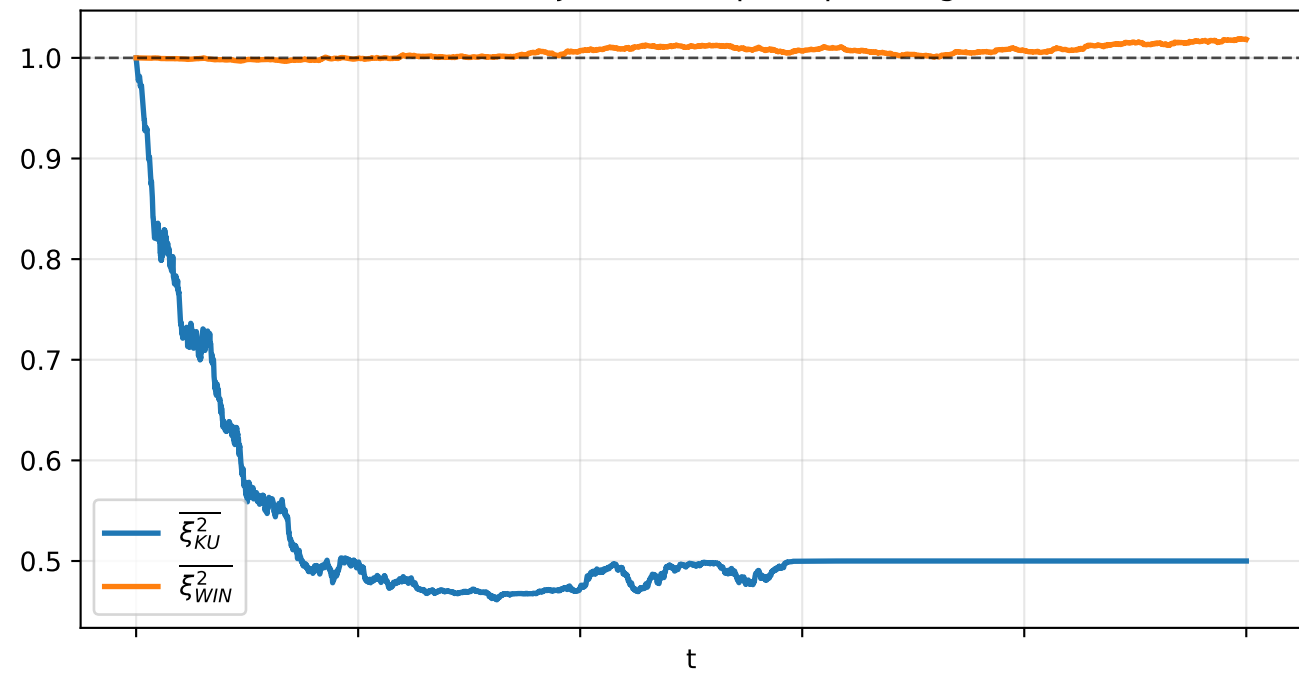
Ideal trajectories: Variance on J_z
