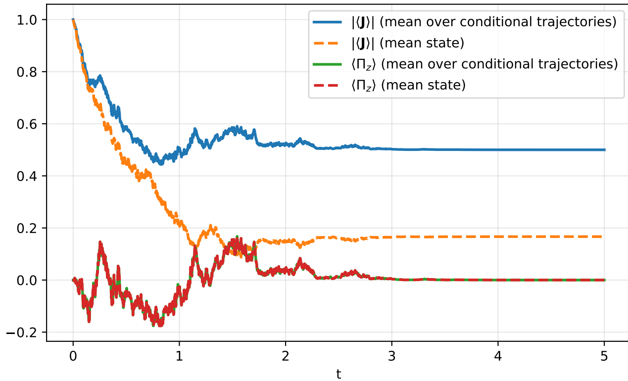
Mixed monitoring: norm and parity
