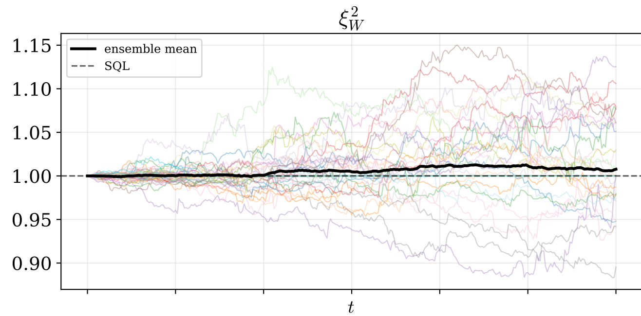
Ideal trajectories ( \eta=1 , ntraj = 50, \phi_1=0 , \phi_2=0 )
