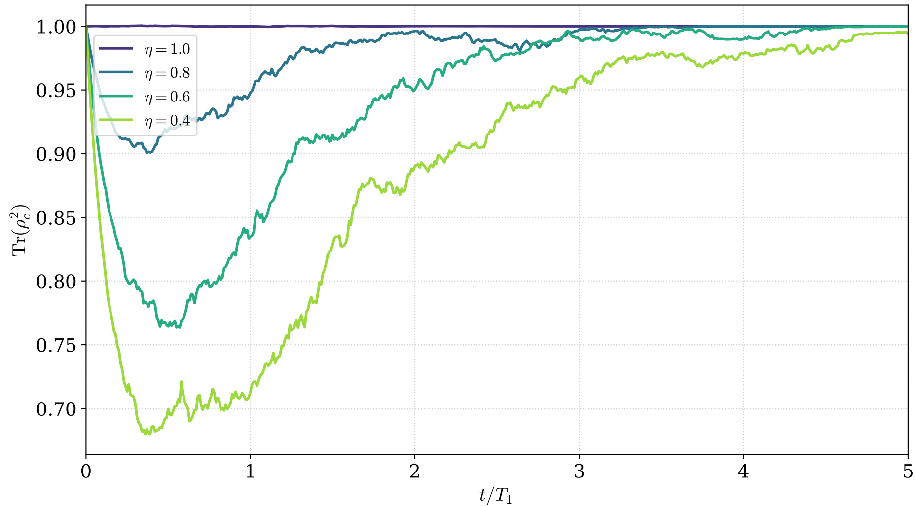
Efficiency scan — \text{Tr}(\rho_c^2) (ntraj = 50, \phi_1 = 0 , \phi_2 = 0 )
