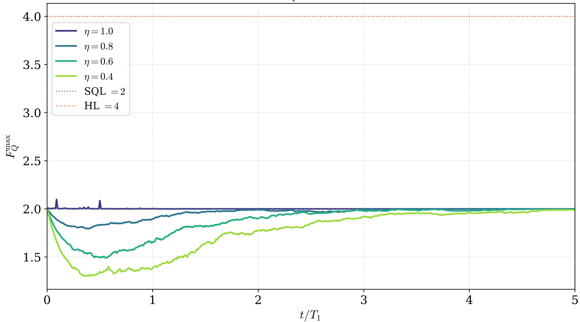
Efficiency scan — F_Q^{\max} (ntraj = 50, \phi_1 = 0 , \phi_2 = 0 )
