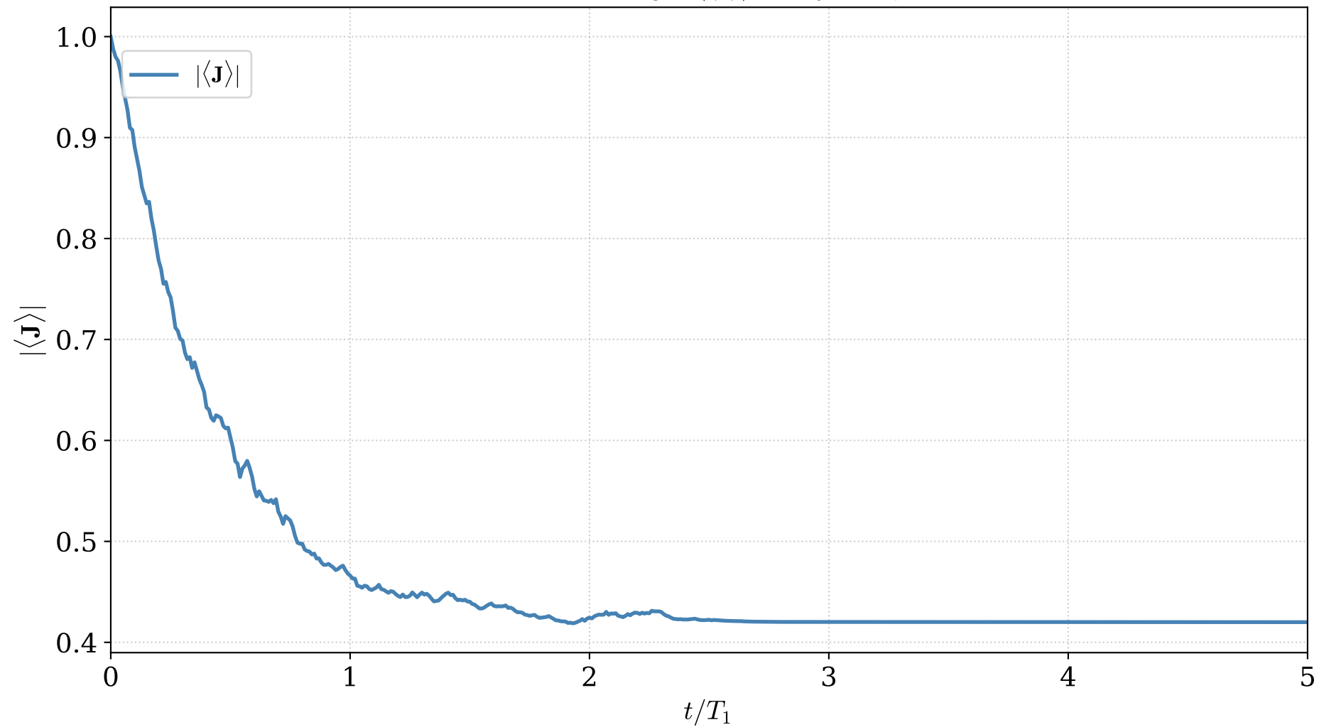
Ideal monitoring — |\langle \mathbf{J} \rangle| (ntraj = 50, \eta = 1 )
