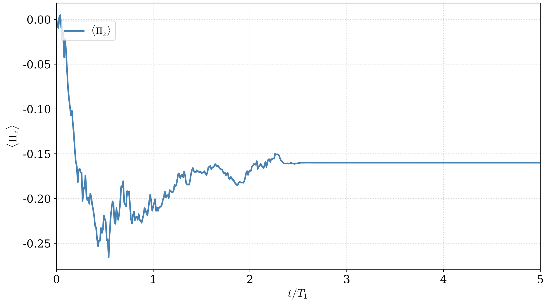
Ideal monitoring — \langle \Pi_z \rangle (ntraj = 50, \eta = 1 )
