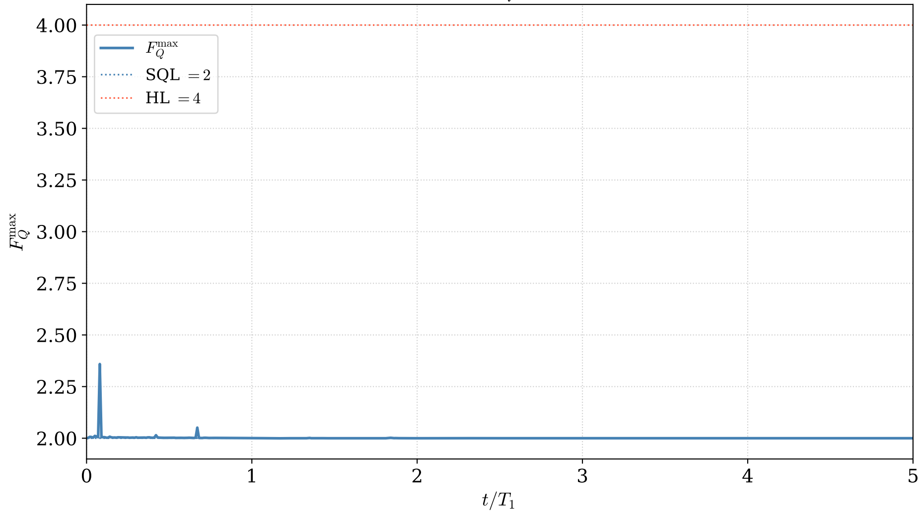
Ideal monitoring — F_Q^{\max} (ntraj = 50, \eta = 1 )
