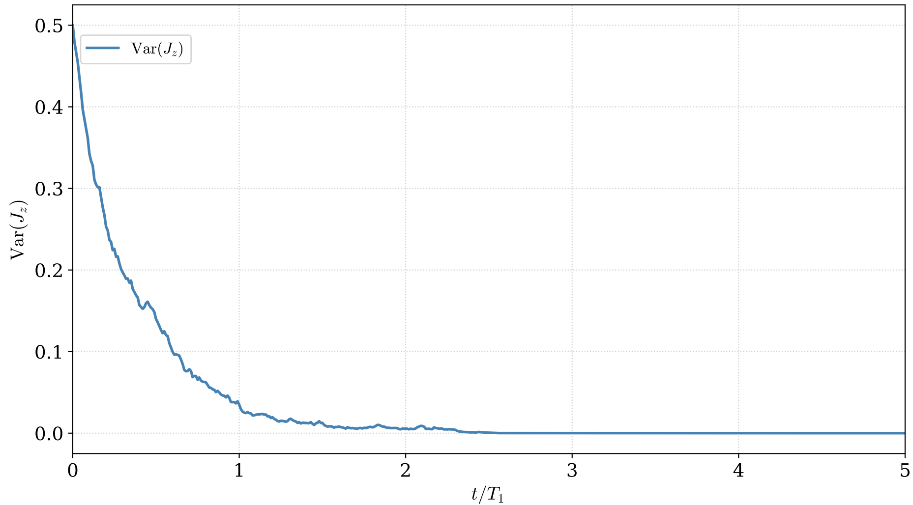
Ideal monitoring — \text{Var}(J_z) (ntraj = 50, \eta = 1 )
