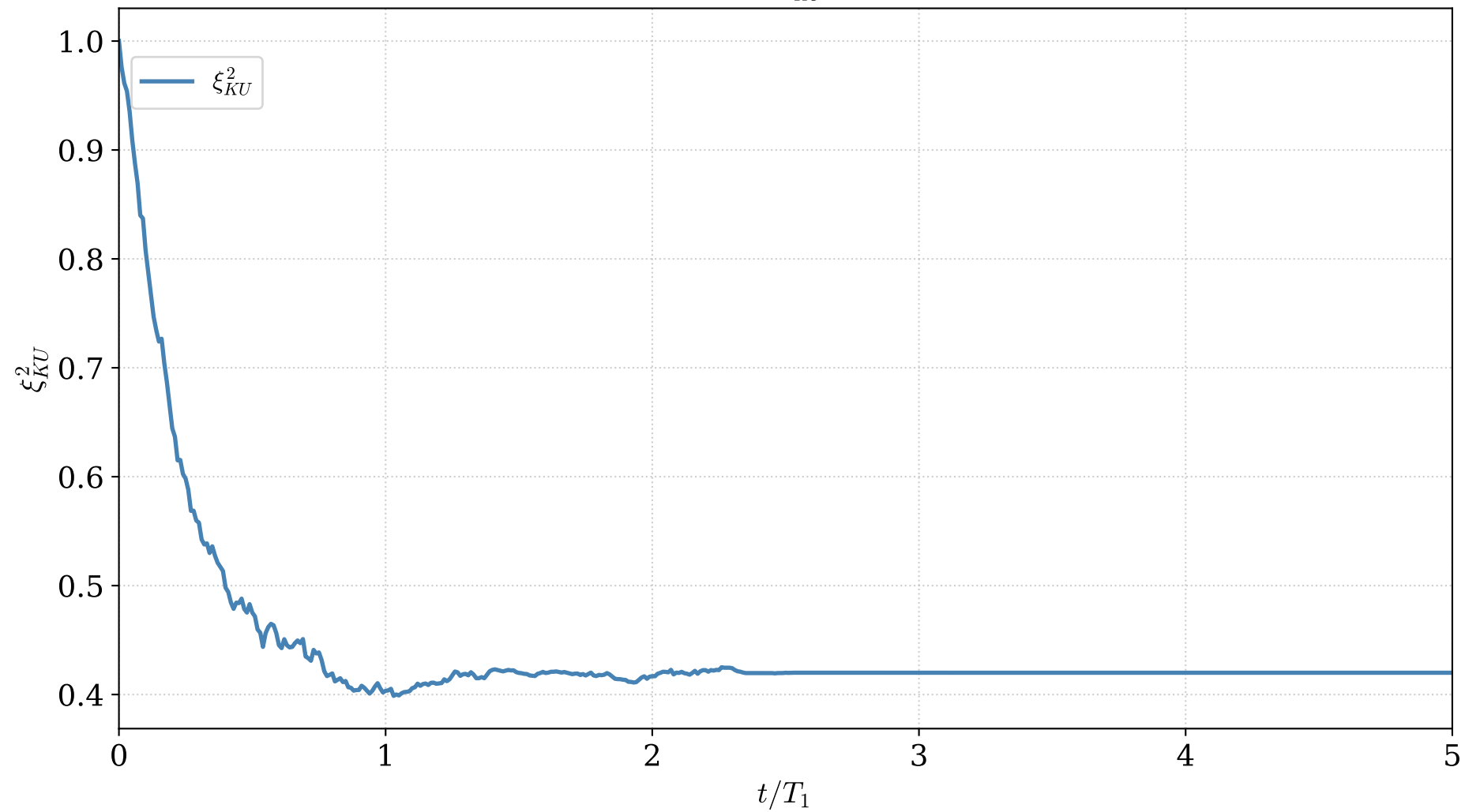
Ideal monitoring — \xi_{KU}^2 (ntraj = 50, \eta = 1 )
