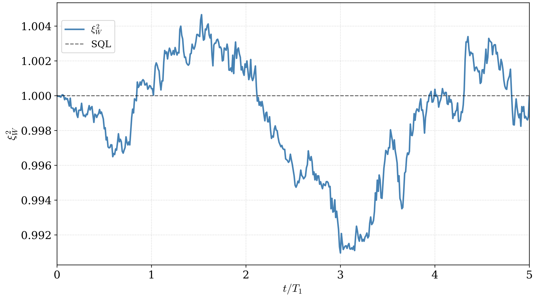
Ideal monitoring — \xi_W^2 (ntraj = 50, \eta = 1 )
