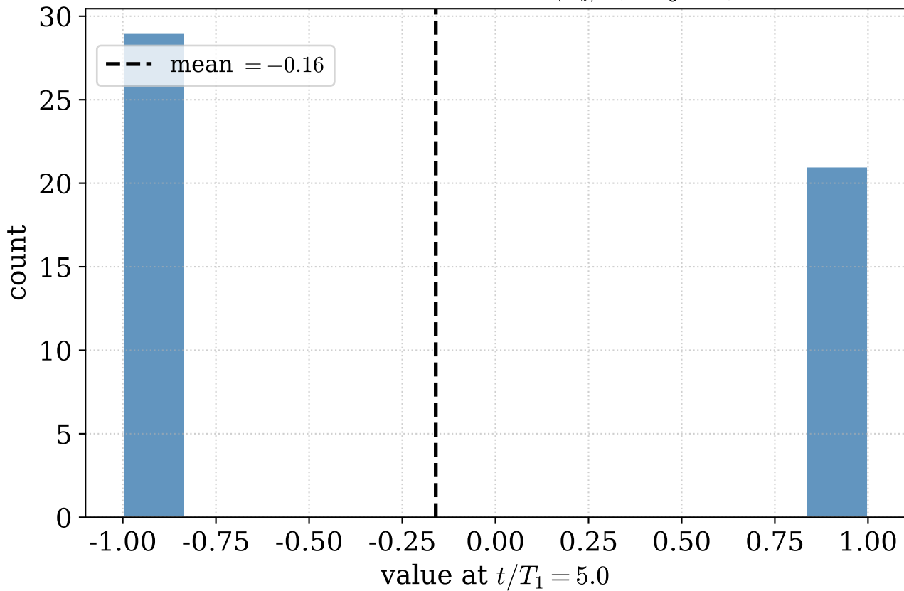
Final-time distribution — \langle \Pi_z \rangle (ntraj = 50)
