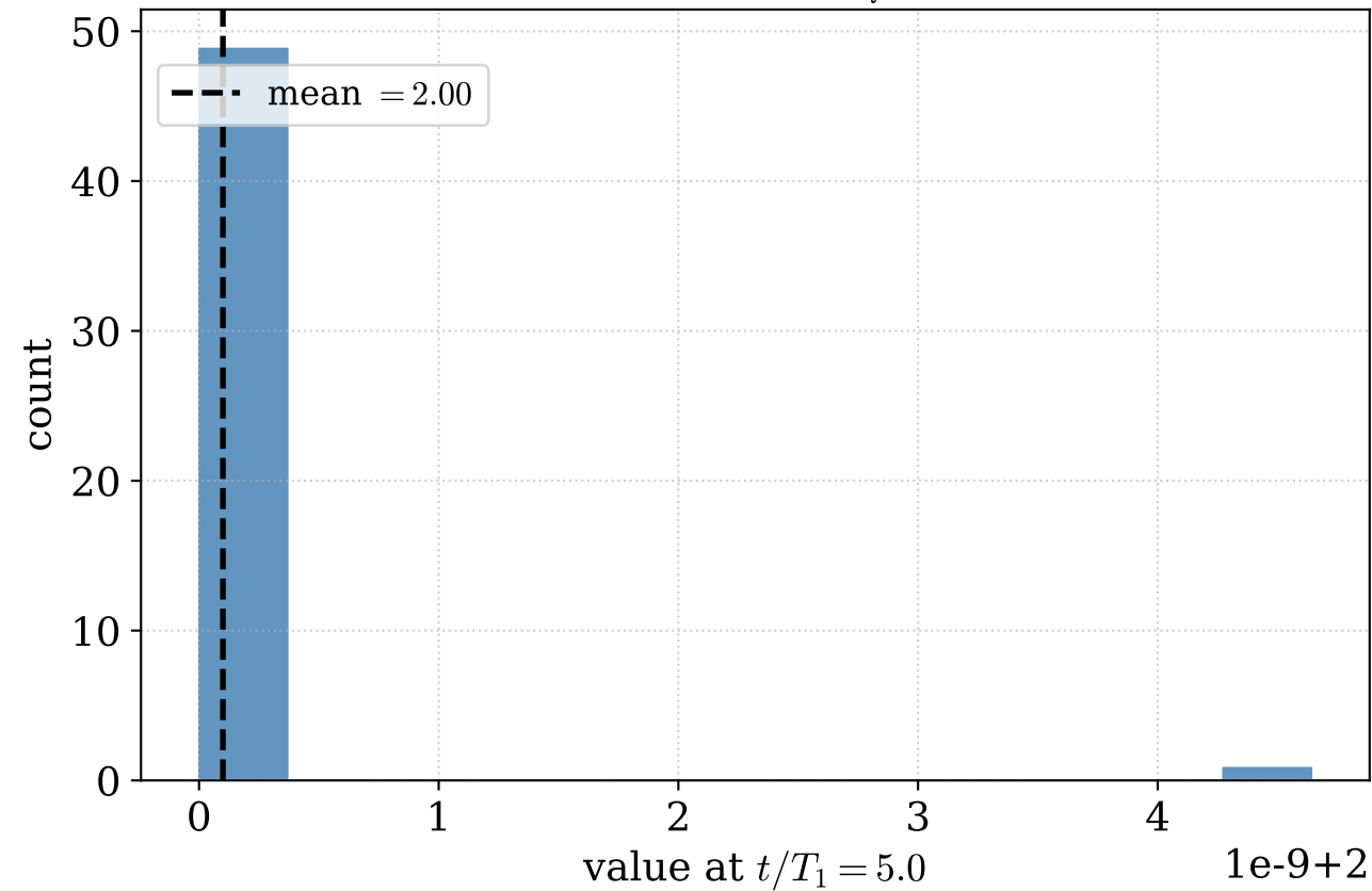
Final-time distribution — F_Q^{\max} (ntraj = 50)
