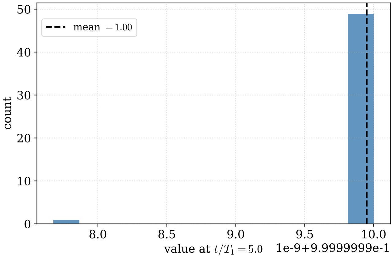
Final-time distribution — \chi^2 (ntraj = 50)
