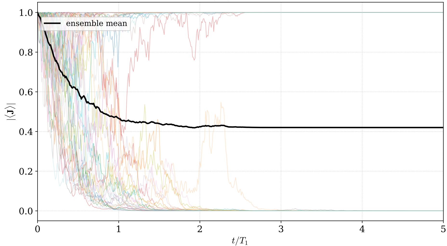
Ideal trajectories — |\langle \mathbf{J} \rangle| ( \eta = 1 , \text{ntraj} = 50 , \phi_1 = 0 , \phi_2 = 0 )
