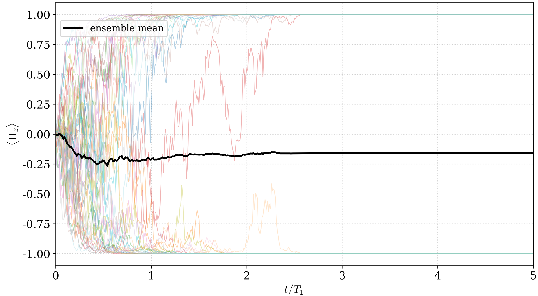
Ideal trajectories — \langle \Pi_z \rangle ( \eta = 1 , ntraj = 50, \phi_1 = 0 , \phi_2 = 0 )
