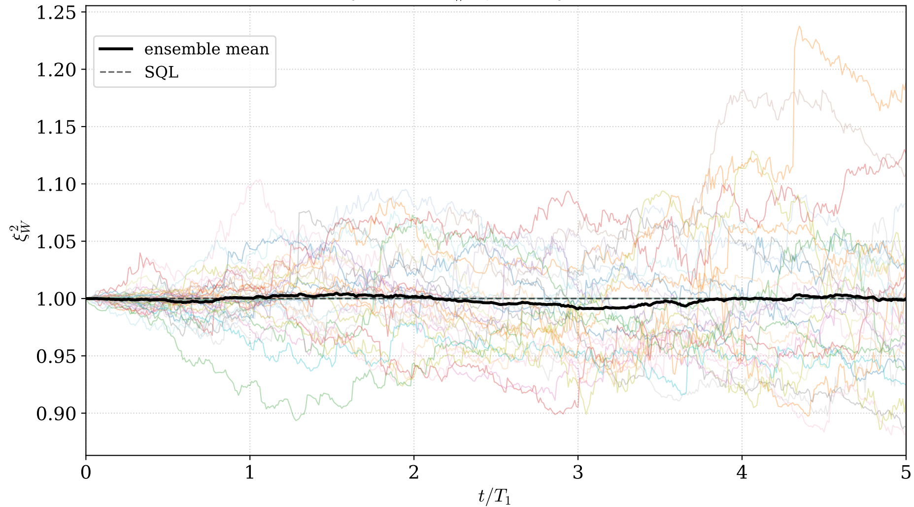
Ideal trajectories — \xi_W^2 ( \eta = 1 , ntraj = 50, \phi_1 = 0 , \phi_2 = 0 )
