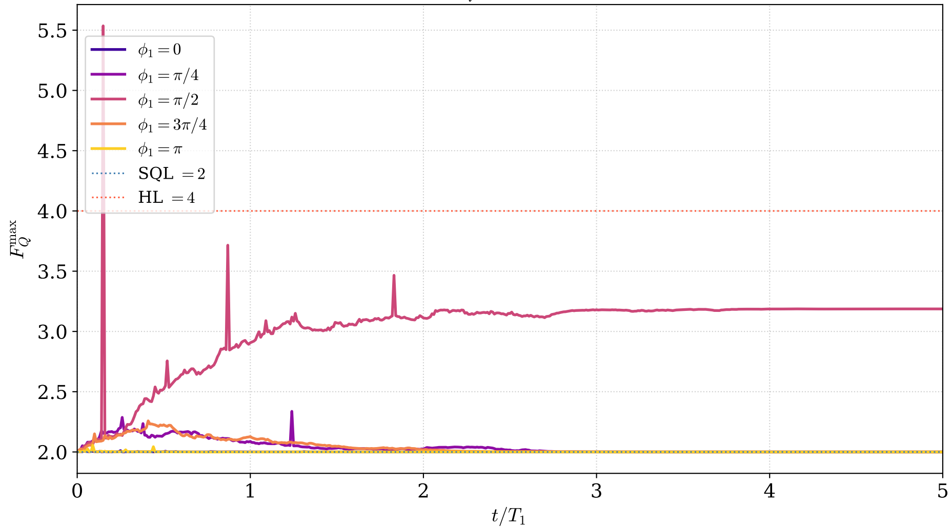
Phase scan — F_Q^{\max} ( \phi_2 = 0 , \eta = 1 , ntraj = 50)
