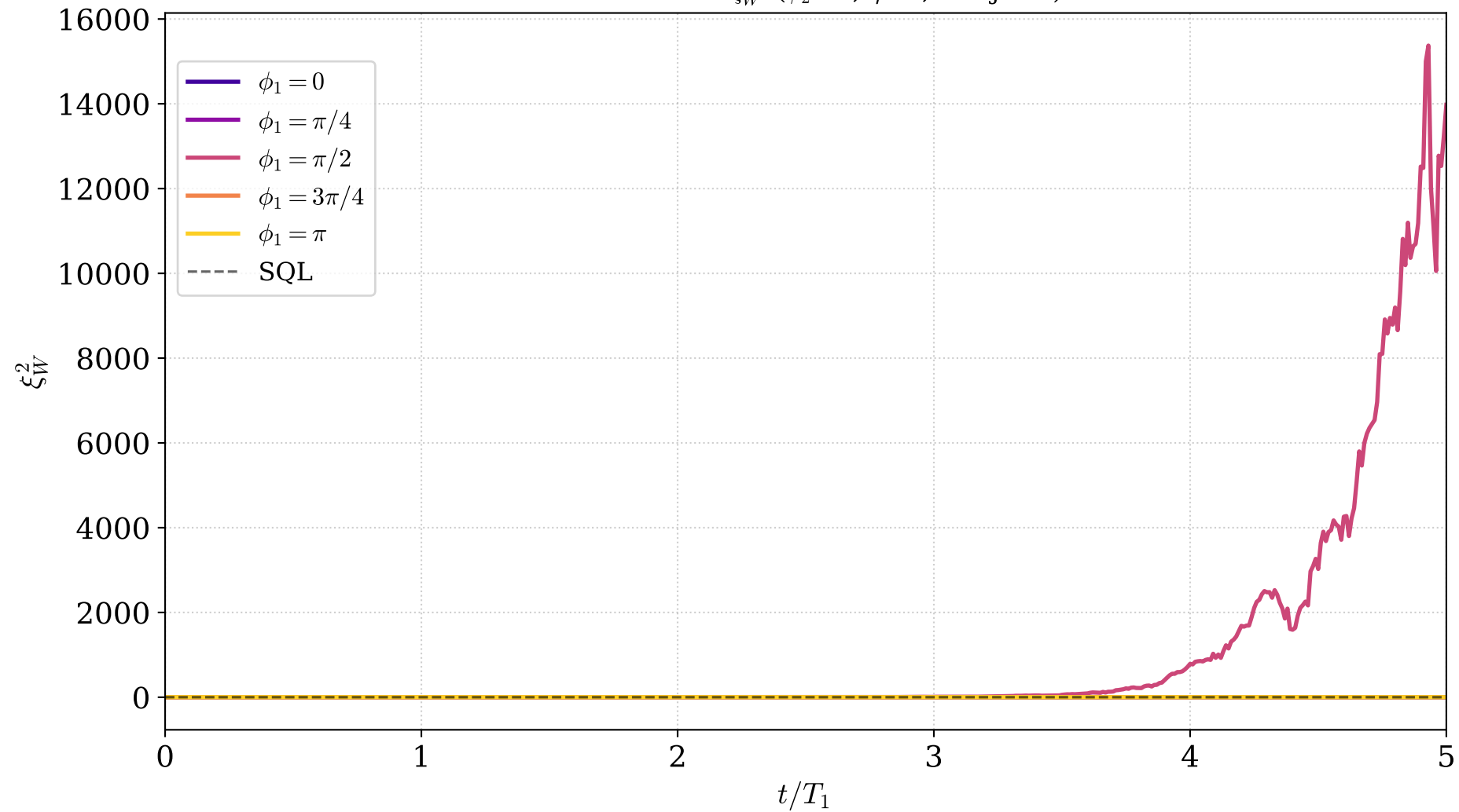
Phase scan — \xi_W^2 ( \phi_2 = 0 , \eta = 1 , ntraj = 50)
