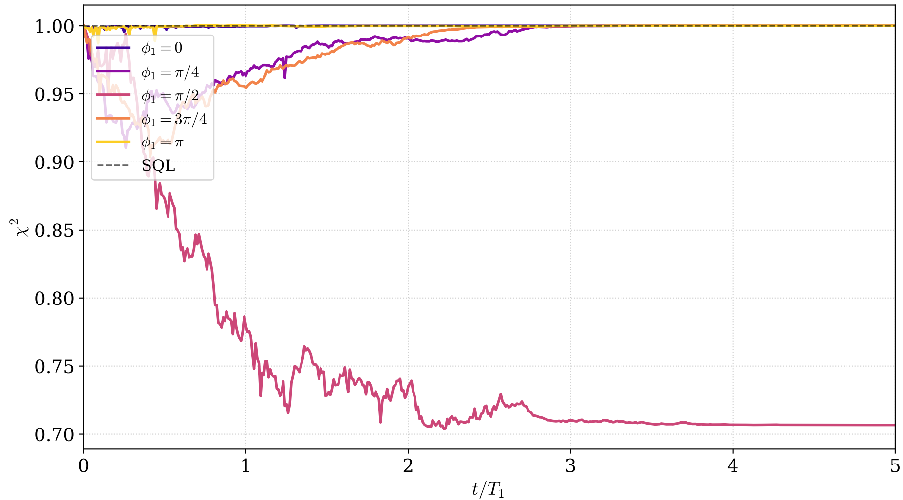
Phase scan — \chi^2 ( \phi_2 = 0 , \eta = 1 , ntraj = 50)
