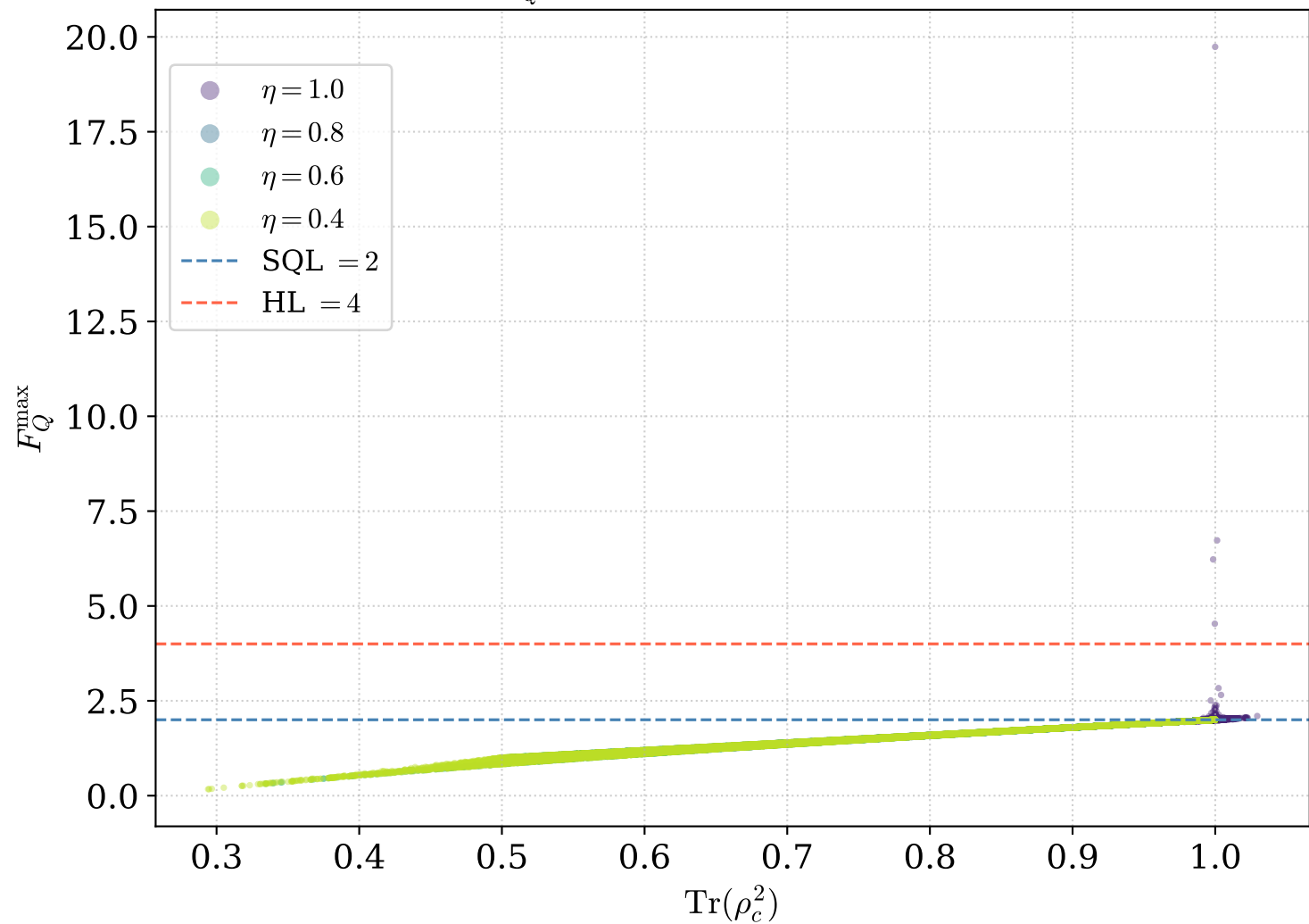
F_Q^{\max} vs purity — all trajectories
