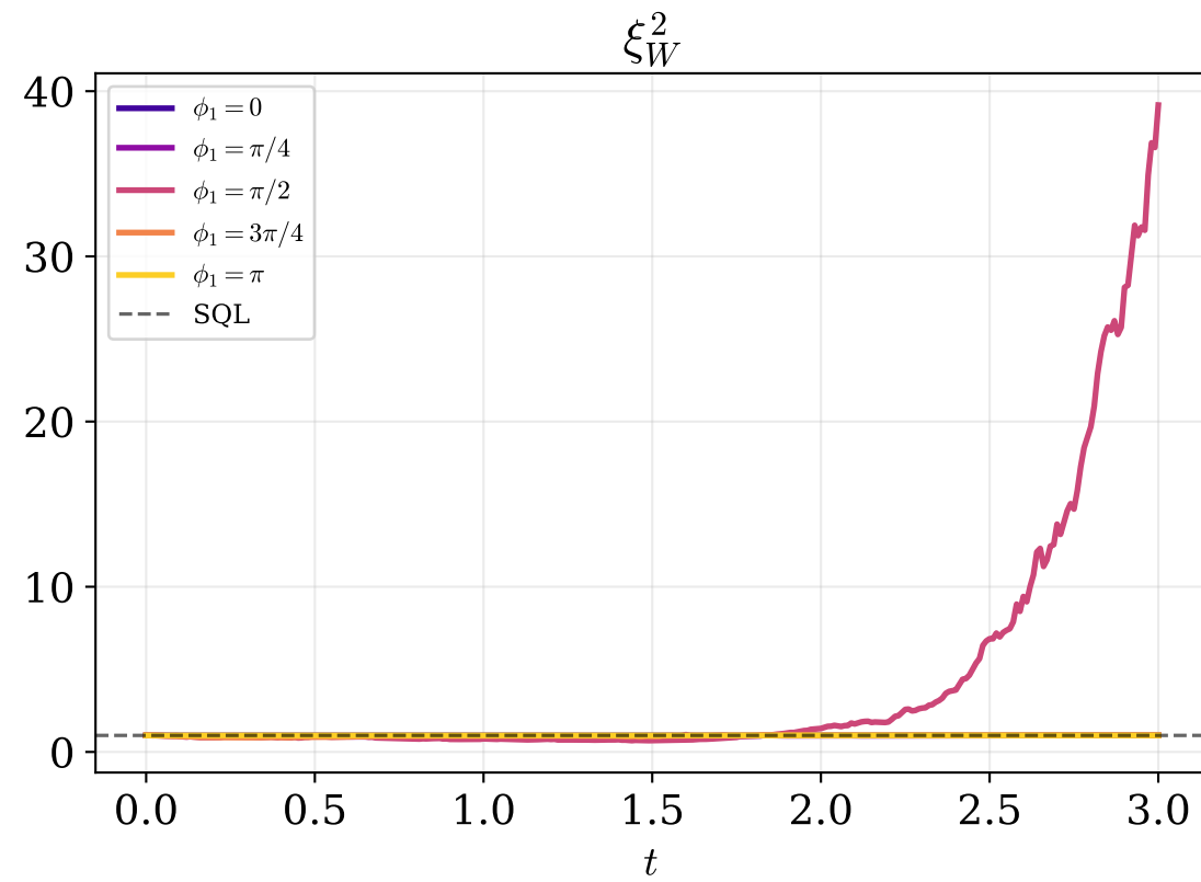
Phase scan: \phi_2 = 0 , \eta = 1 , ntraj = 20
