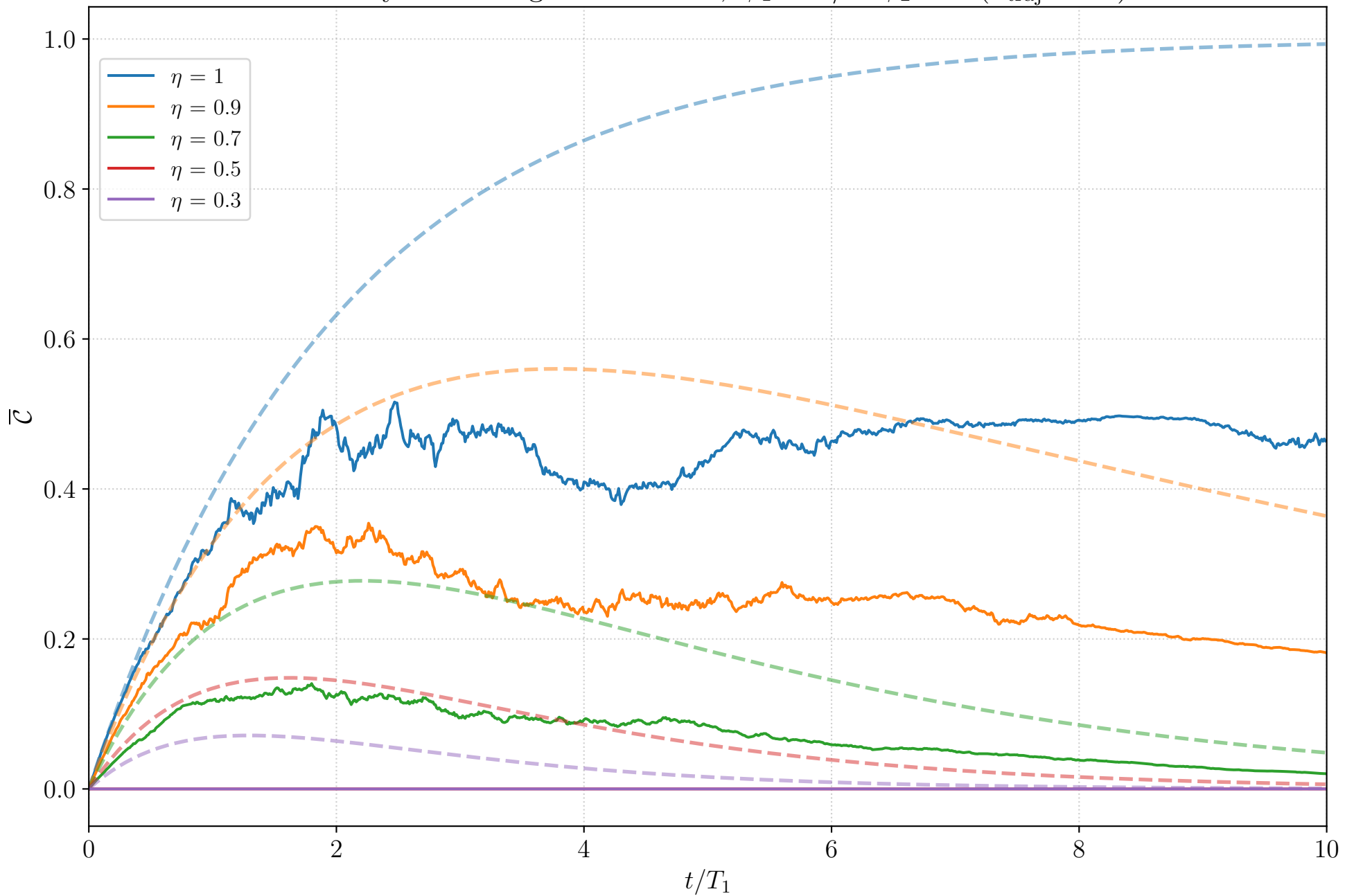
Homodyne: Average \bar{\mathcal{C}} over time, \phi_1 = \pi/2 \phi_2 = 0 ( n_{\text{traj}} = 10 )
