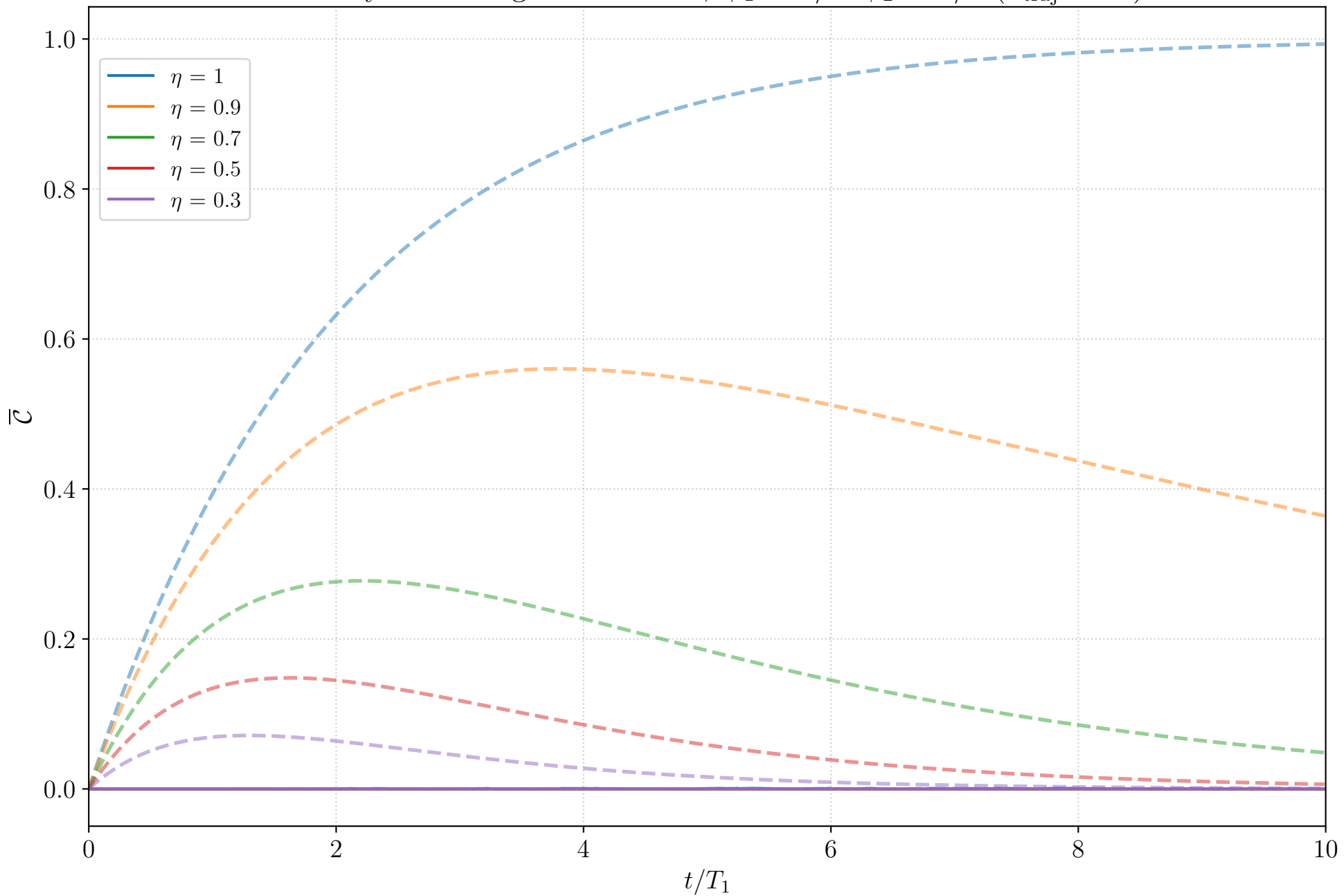
Homodyne: Average \bar{\mathcal{C}} over time, \phi_1 = \pi/2 \phi_2 = \pi/2 ( n_{\text{traj}} = 10 )
