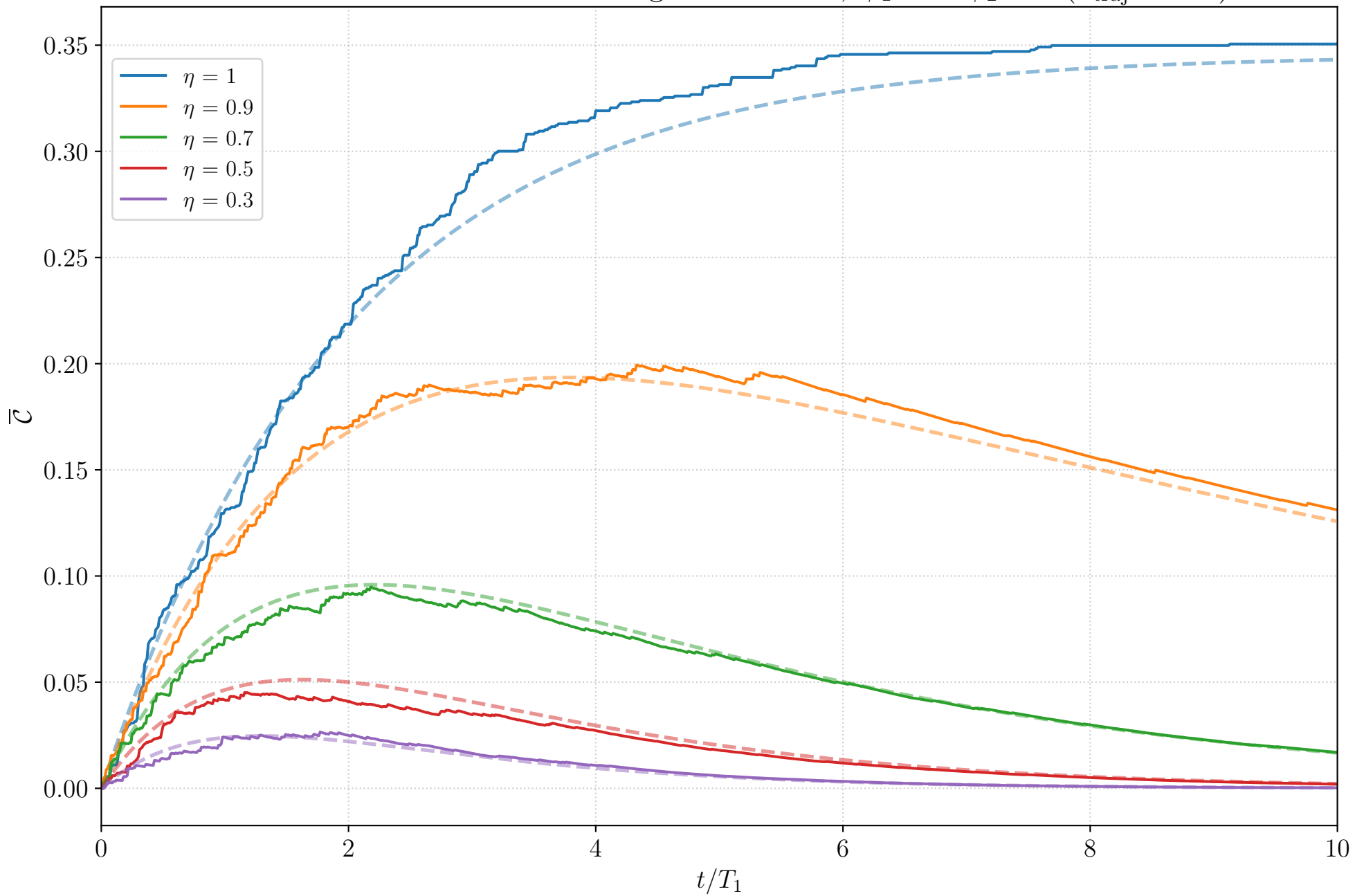
Inefficient Photodetection: Average \bar{\mathcal{C}} over time, \phi_1 = 0 \phi_2 = 0 ( n_{\text{traj}} = 300 )
