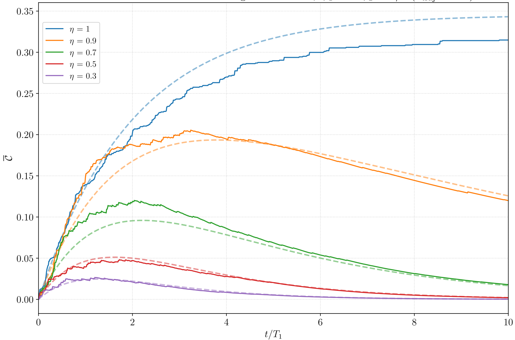
Inefficient Photodetection: Average \overline{\mathcal{C}} over time, \phi_1 = 0 \phi_2 = \pi/2 ( n_{\text{traj}} = 300 )
