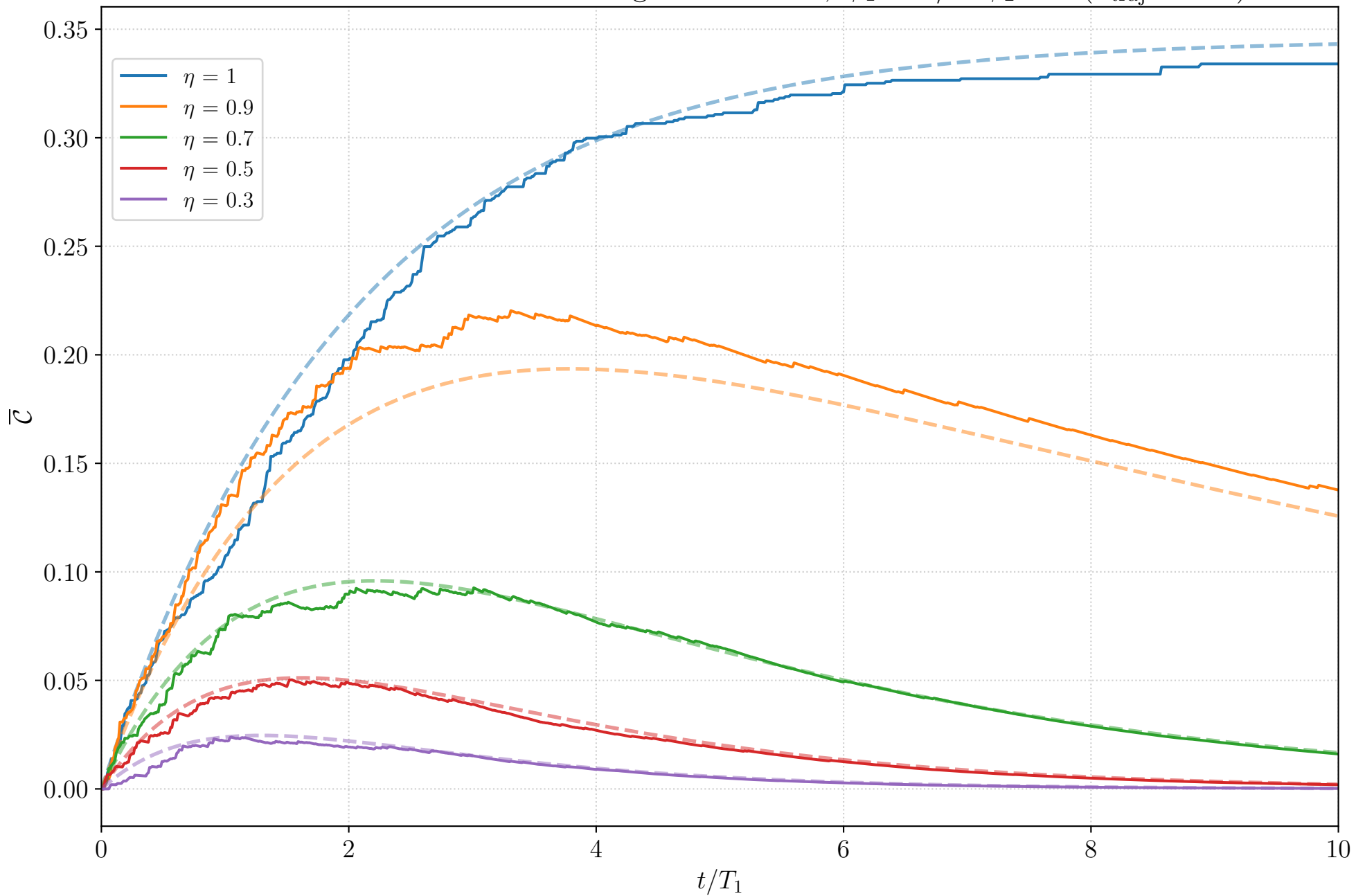
Inefficient Photodetection: Average \overline{\mathcal{C}} over time, \phi_1 = \pi/2 \phi_2 = 0 ( n_{\text{traj}} = 300 )
