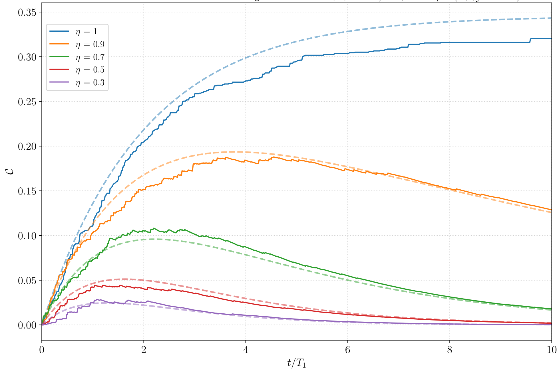
Inefficient Photodetection: Average \bar{\mathcal{C}} over time, \phi_1 = \pi/2 \phi_2 = \pi/2 ( n_{\text{traj}} = 300 )
