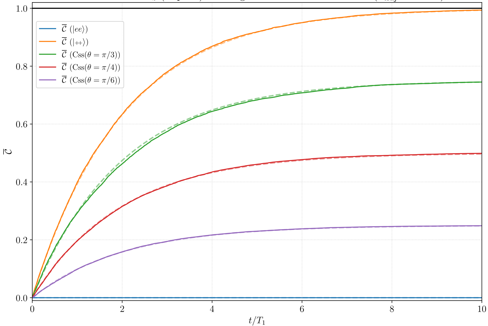
Photodetection J_z (2 qubit): Average concurrence \bar{\mathcal{C}} over time ( n_{\text{traj}} = 10000 )
