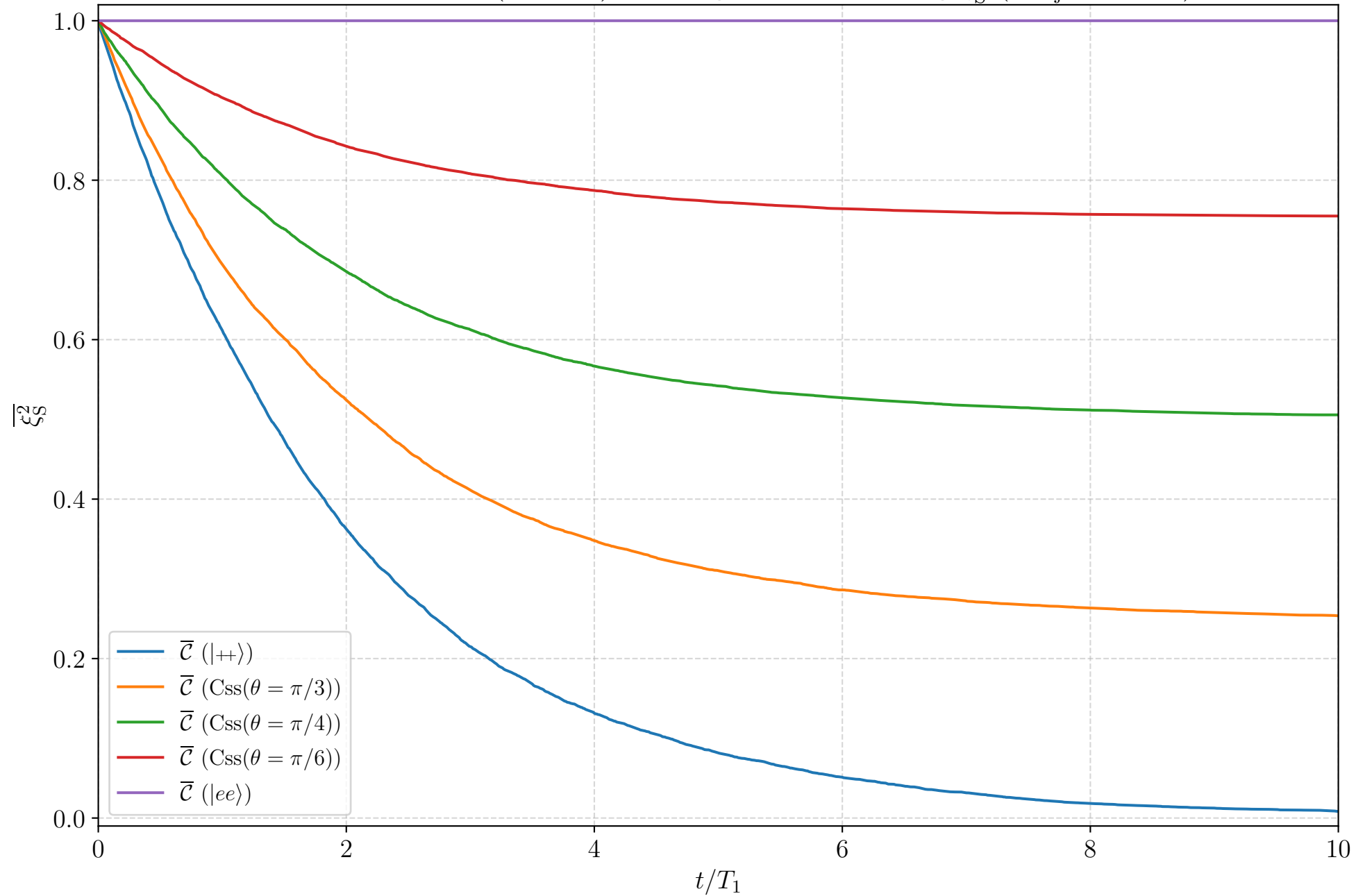
Photodetection J_z (2 qubit): Average Spin Squeezing \overline{\xi_S^2} ( n_{\text{traj}} = 10000 )
