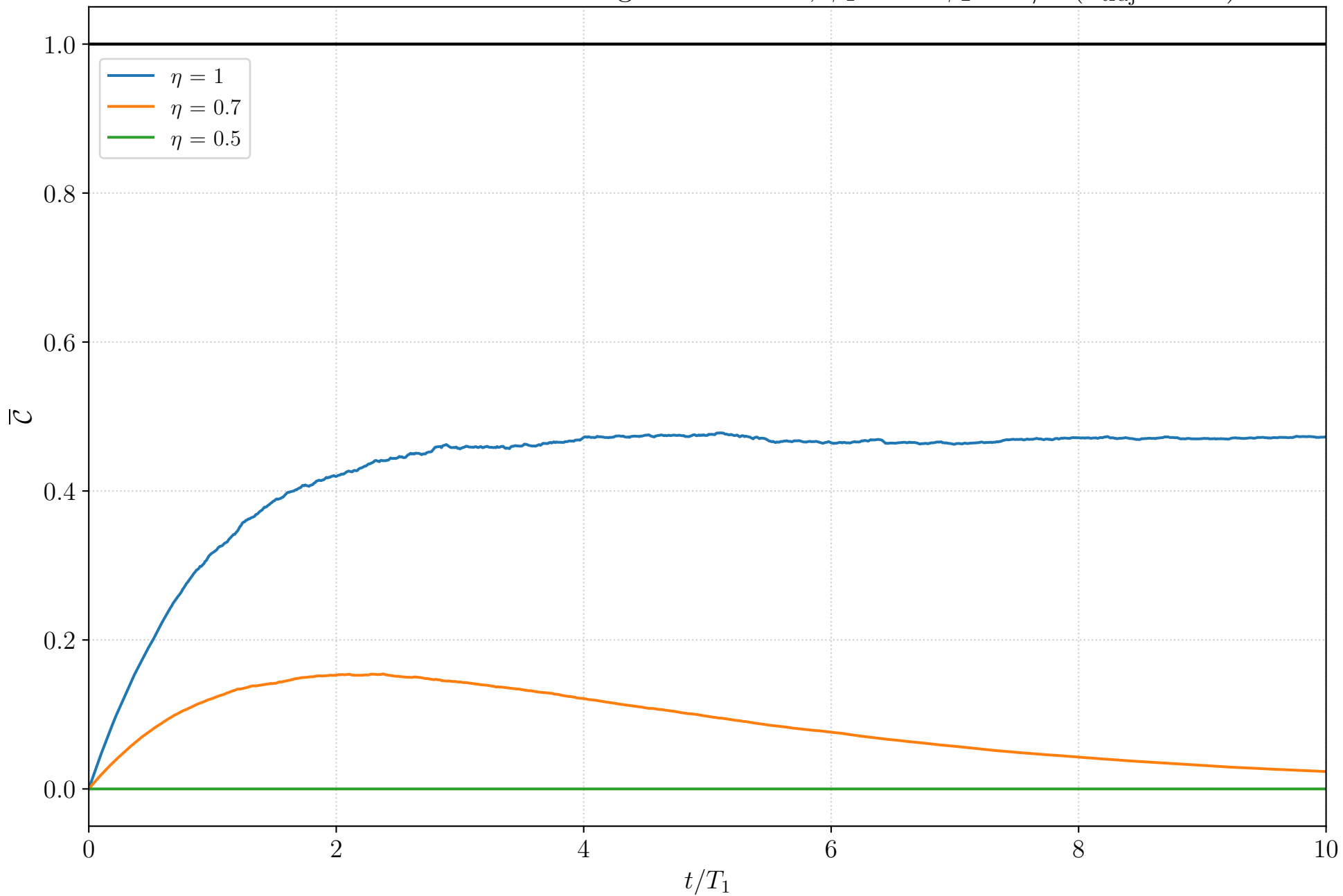
Inefficient Photodetection: Average \bar{\mathcal{C}} over time, \phi_1 = 0 \phi_2 = \pi/2 ( n_{\text{traj}} = 500 )
