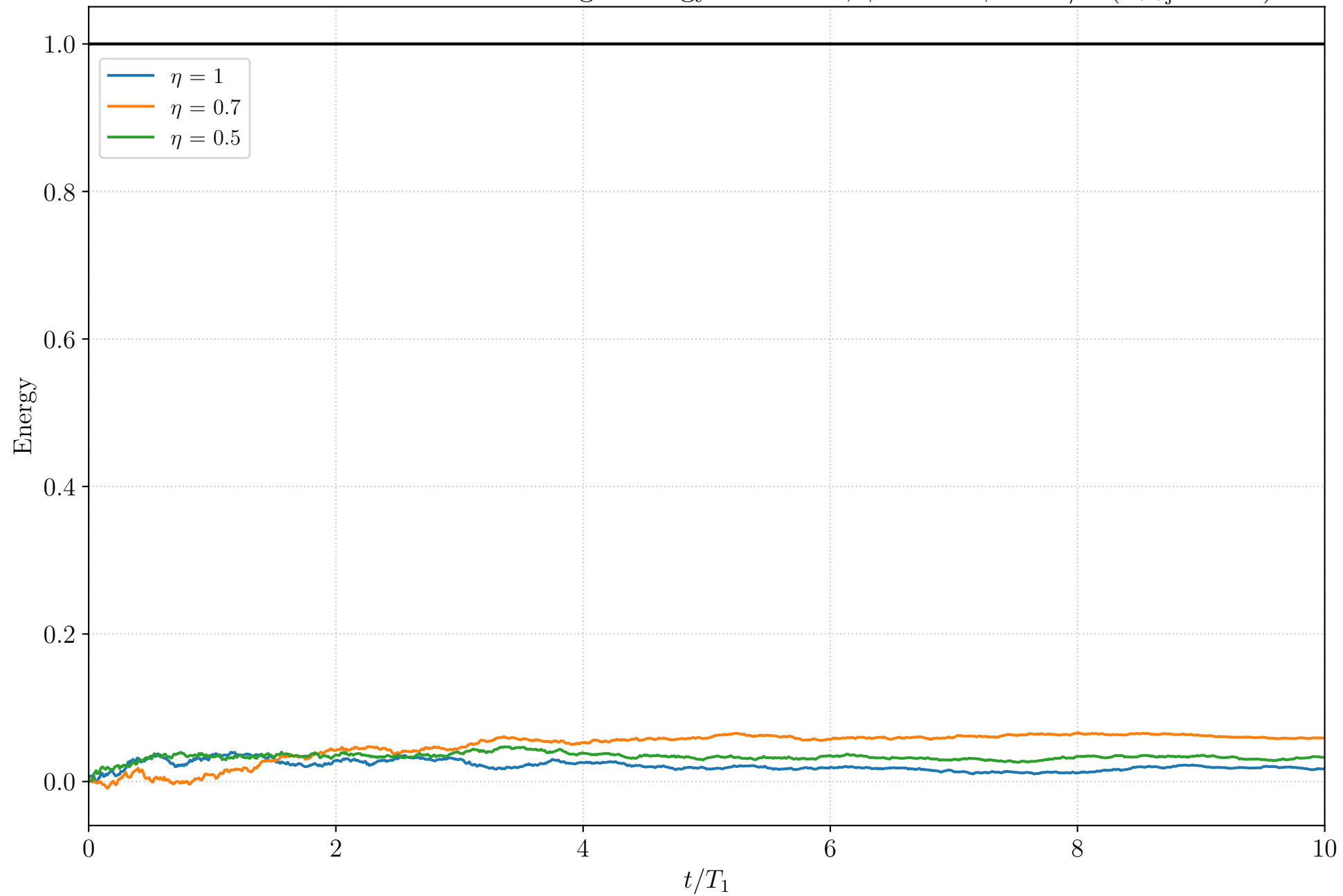
Inefficient Photodetection: Average Energy over time, \phi_1 = 0 \phi_2 = \pi/2 ( n_{\text{traj}} = 500 )
