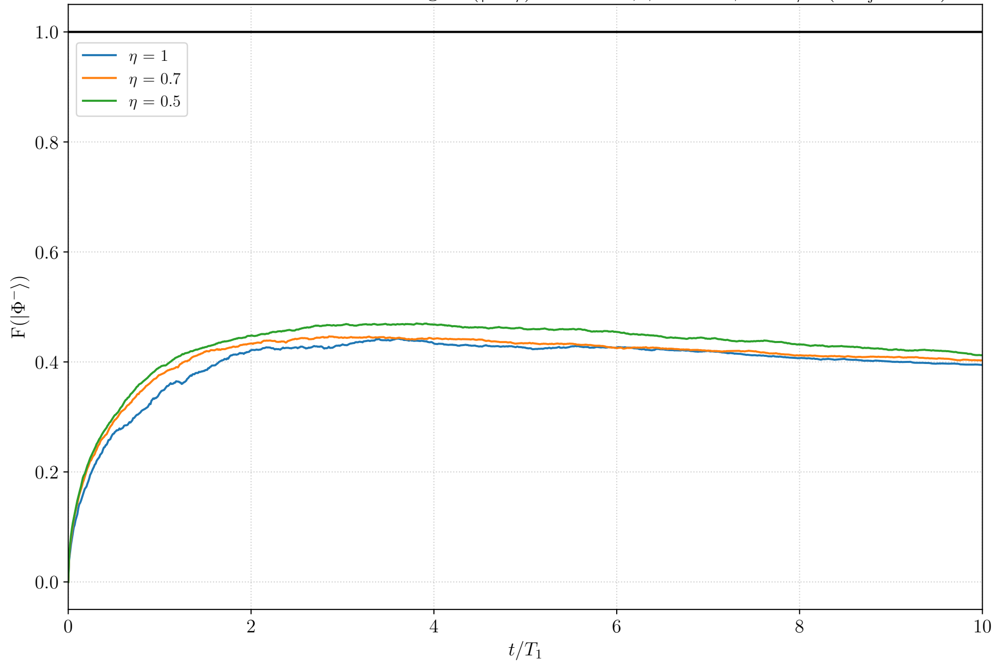
Inefficient Photodetection: Average F(|\Phi^-\rangle) over time, \phi_1 = 0 \phi_2 = \pi/2 ( n_{\text{traj}} = 500 )
