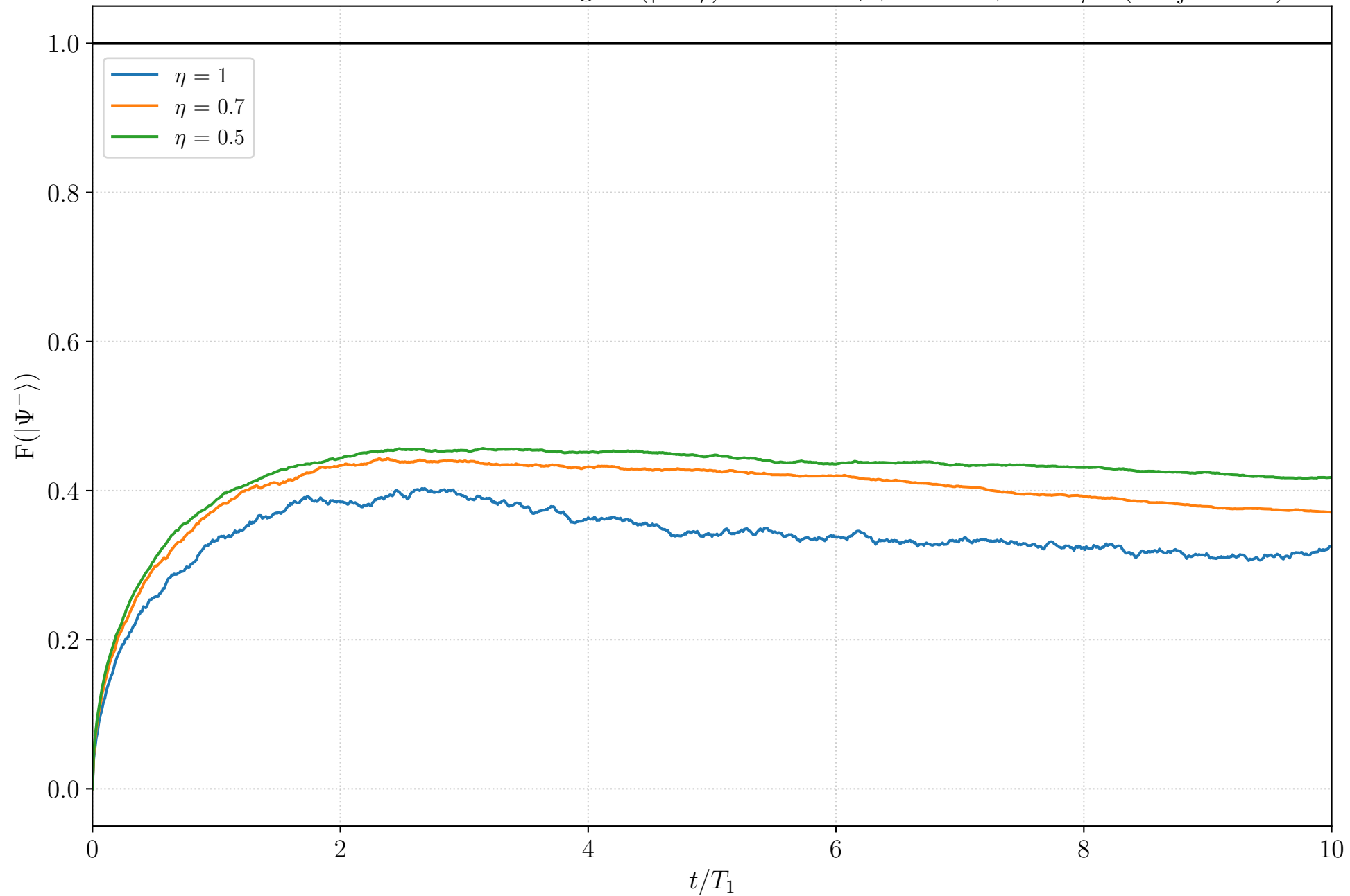
Inefficient Photodetection: Average F(|\Psi^-\rangle) over time, \phi_1 = 0 \phi_2 = \pi/2 ( n_{\text{traj}} = 500 )
