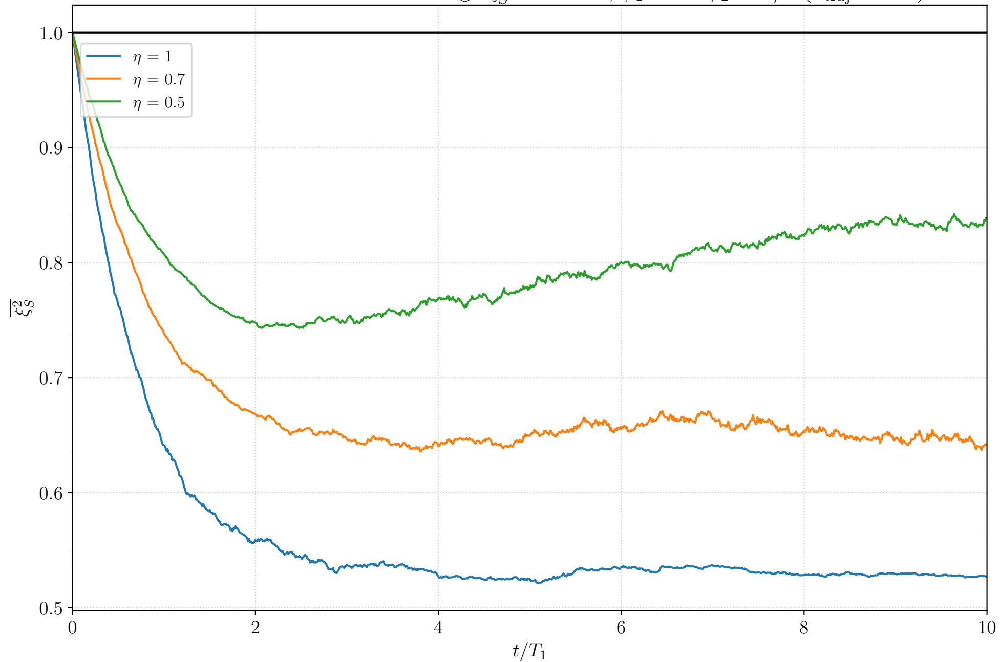
Inefficient Photodetection: Average \overline{\xi_S^2} over time, \phi_1 = 0 \phi_2 = \pi/2 ( n_{\text{traj}} = 500 )
