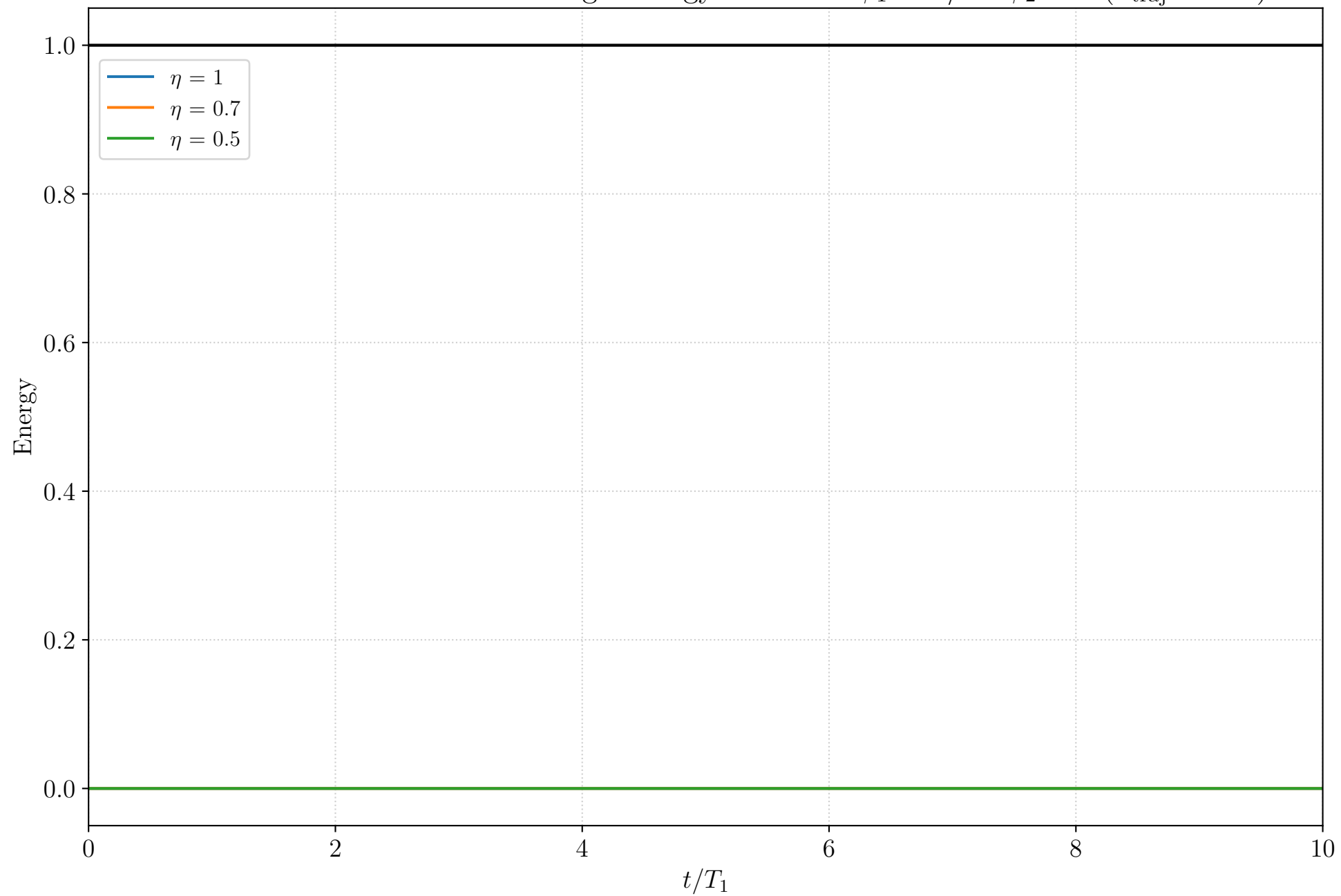
Inefficient Photodetection: Average Energy over time \phi_1 = \pi/2 \phi_2 = 0 ( n_{\text{traj}} = 500 )
