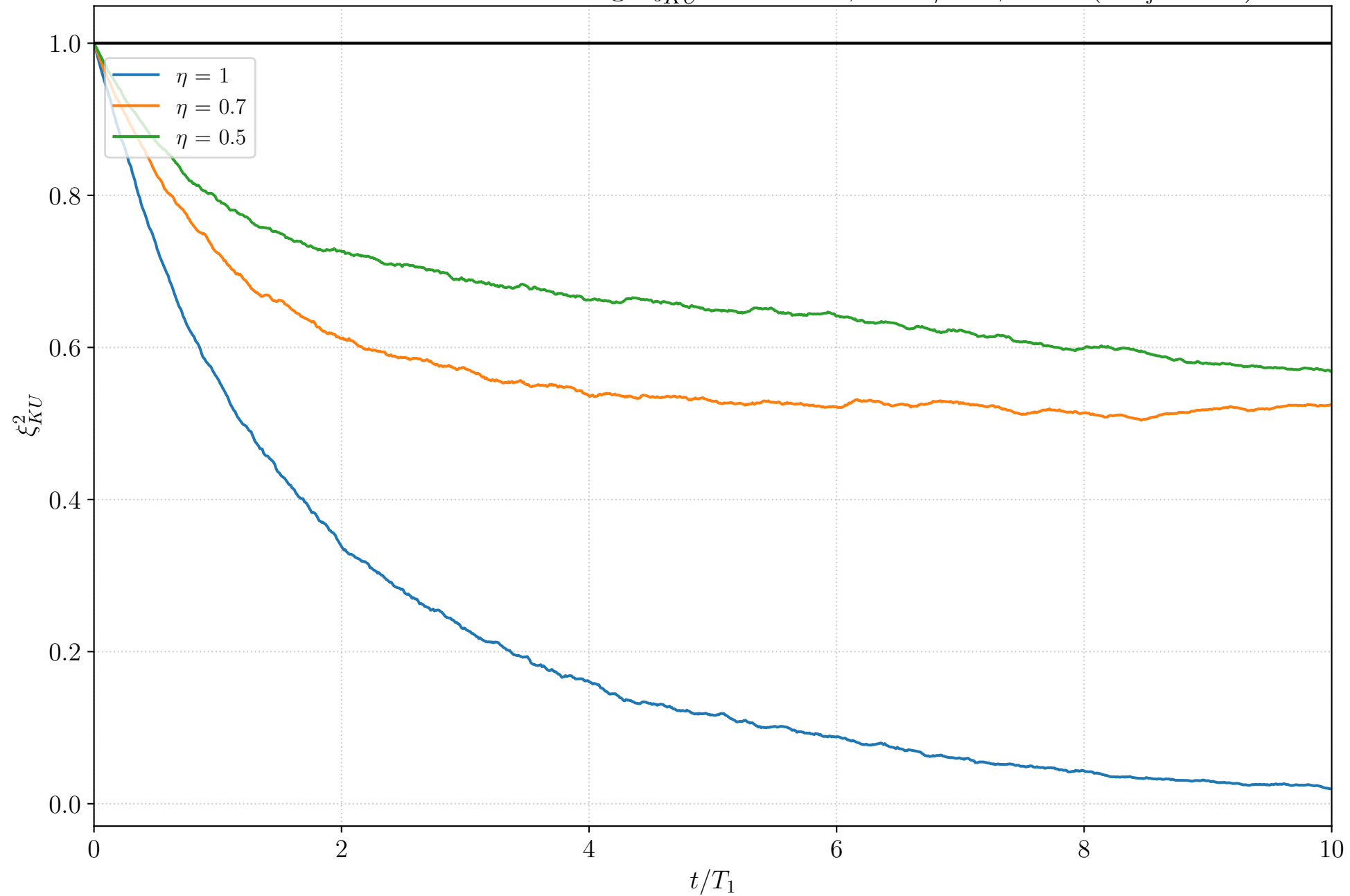
Inefficient Photodetection: Average \xi_{KU}^2 over time \phi_1 = \pi/2 \phi_2 = 0 ( n_{\text{traj}} = 500 )
