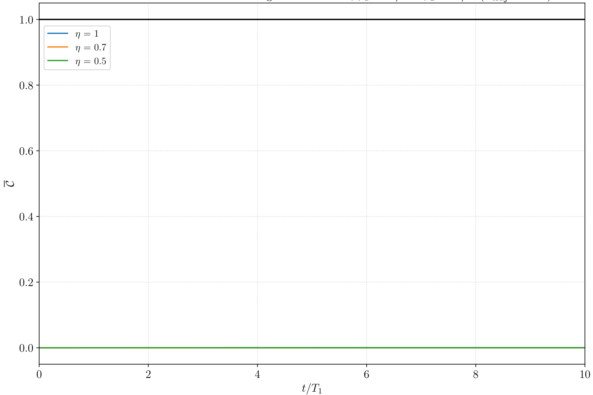
Inefficient Photodetection: Average \overline{\mathcal{C}} over time, \phi_1 = \pi/2 \phi_2 = \pi/2 ( n_{\text{traj}} = 500 )
