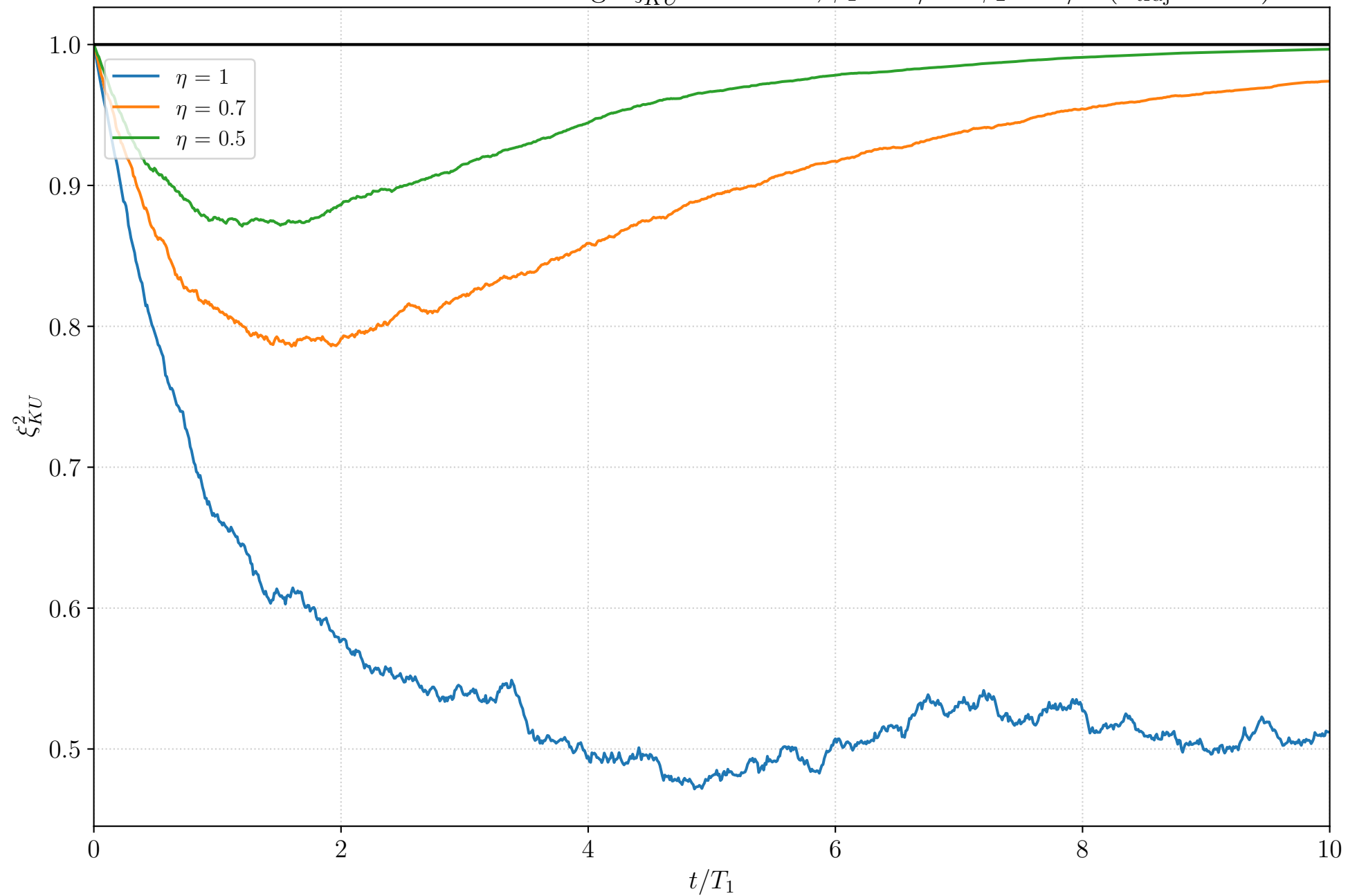
Inefficient Photodetection: Average \xi_{KU}^2 over time, \phi_1 = \pi/2 \phi_2 = \pi/2 ( n_{\text{traj}} = 500 )
