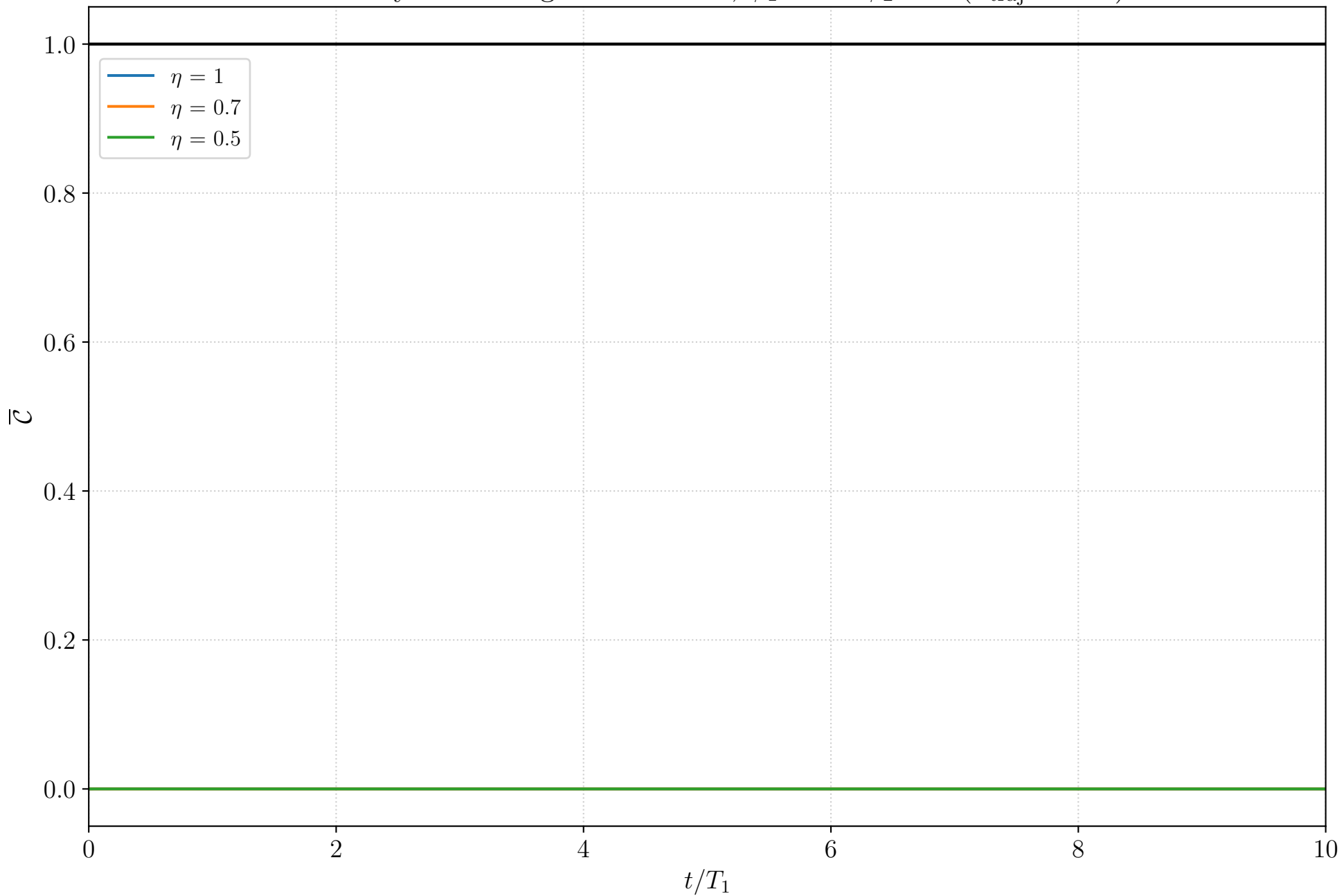
Heterodyne: Average \bar{\mathcal{C}} over time, \phi_1 = 0 \phi_2 = 0 ( n_{\text{traj}} = 100 )
