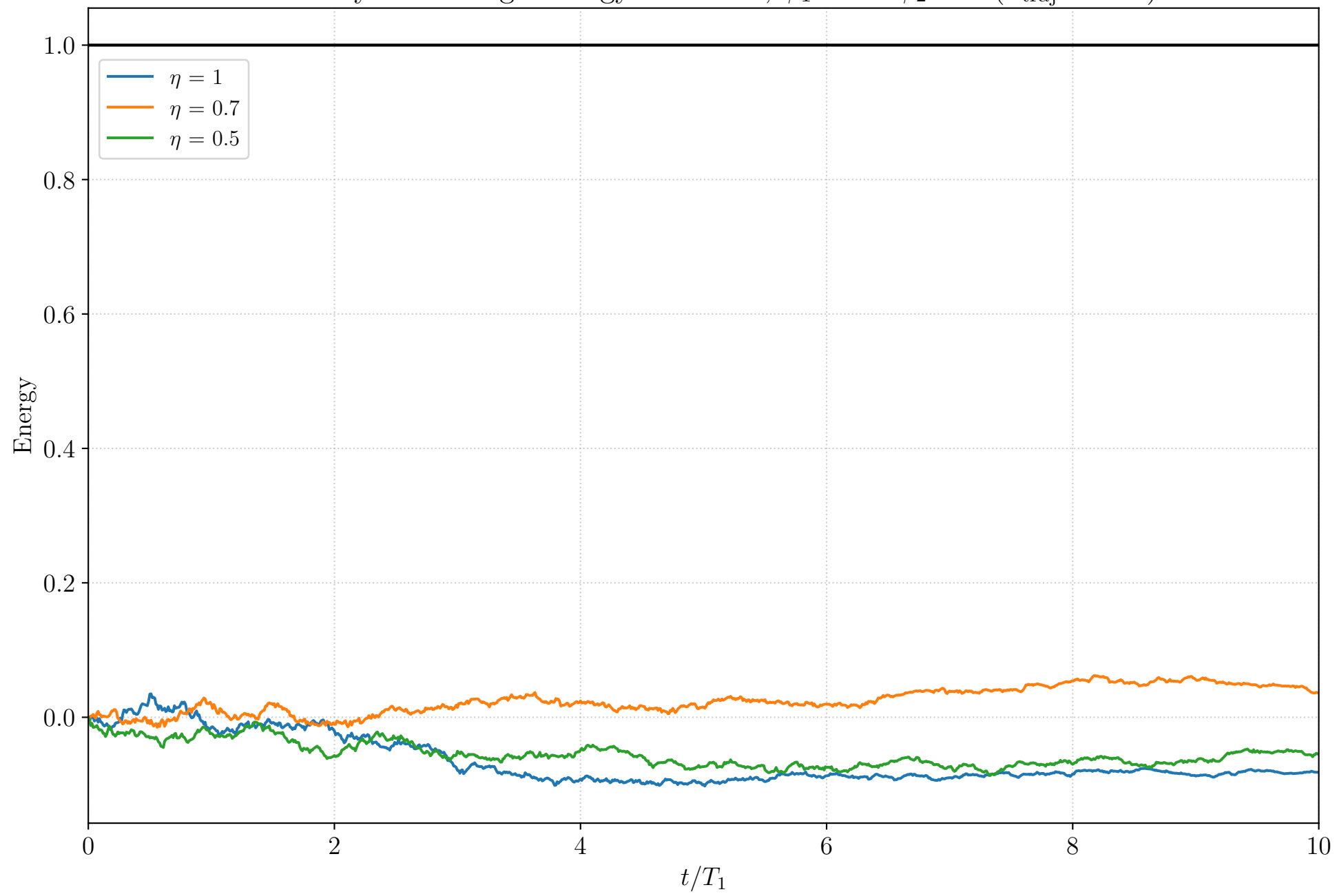
Heterodyne: Average Energy over time, \phi_1 = 0 \phi_2 = 0 ( n_{\text{traj}} = 100 )
