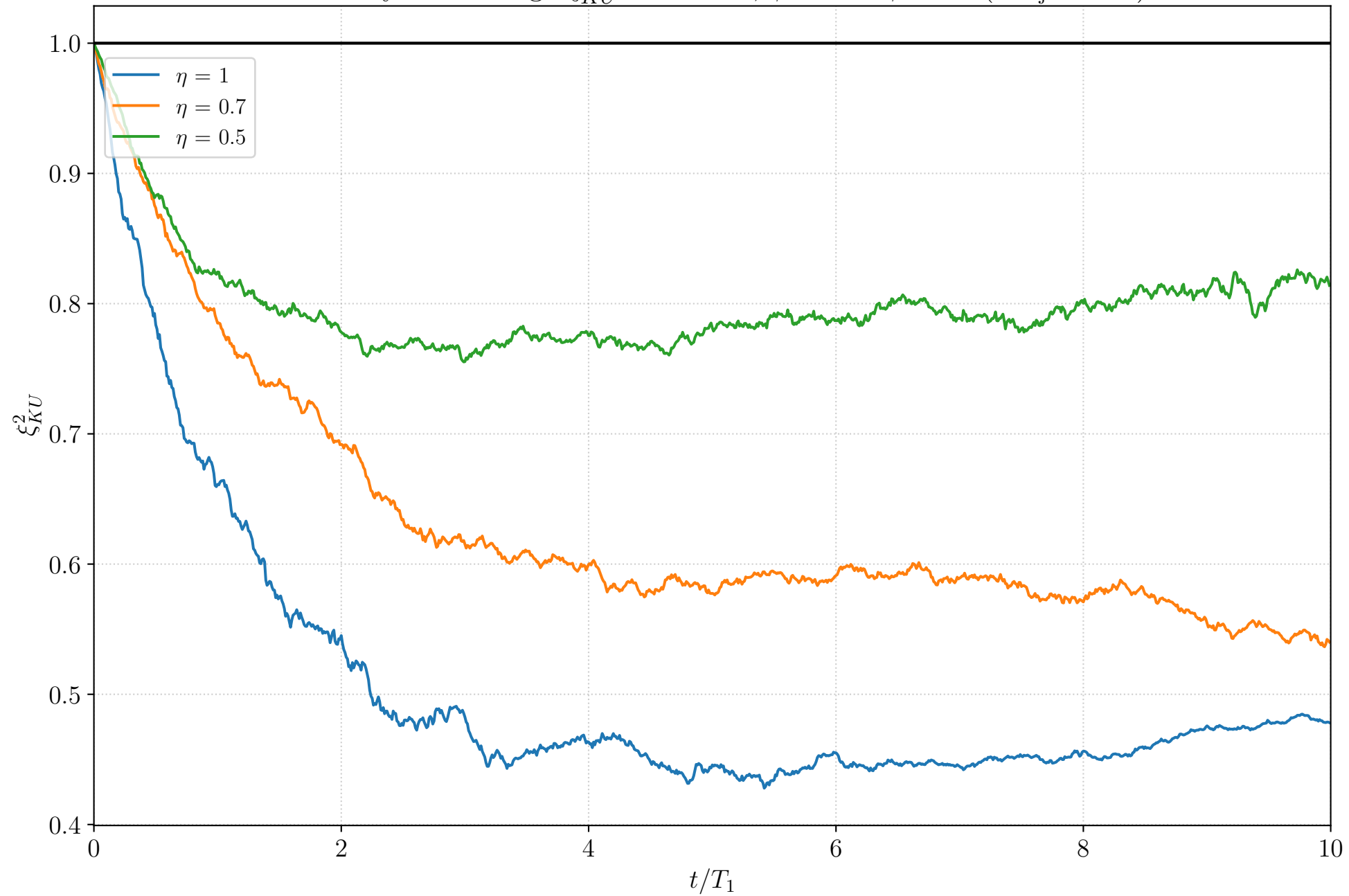
Heterodyne: Average \xi_{KU}^2 over time, \phi_1 = 0 \phi_2 = 0 ( n_{\text{traj}} = 100 )
