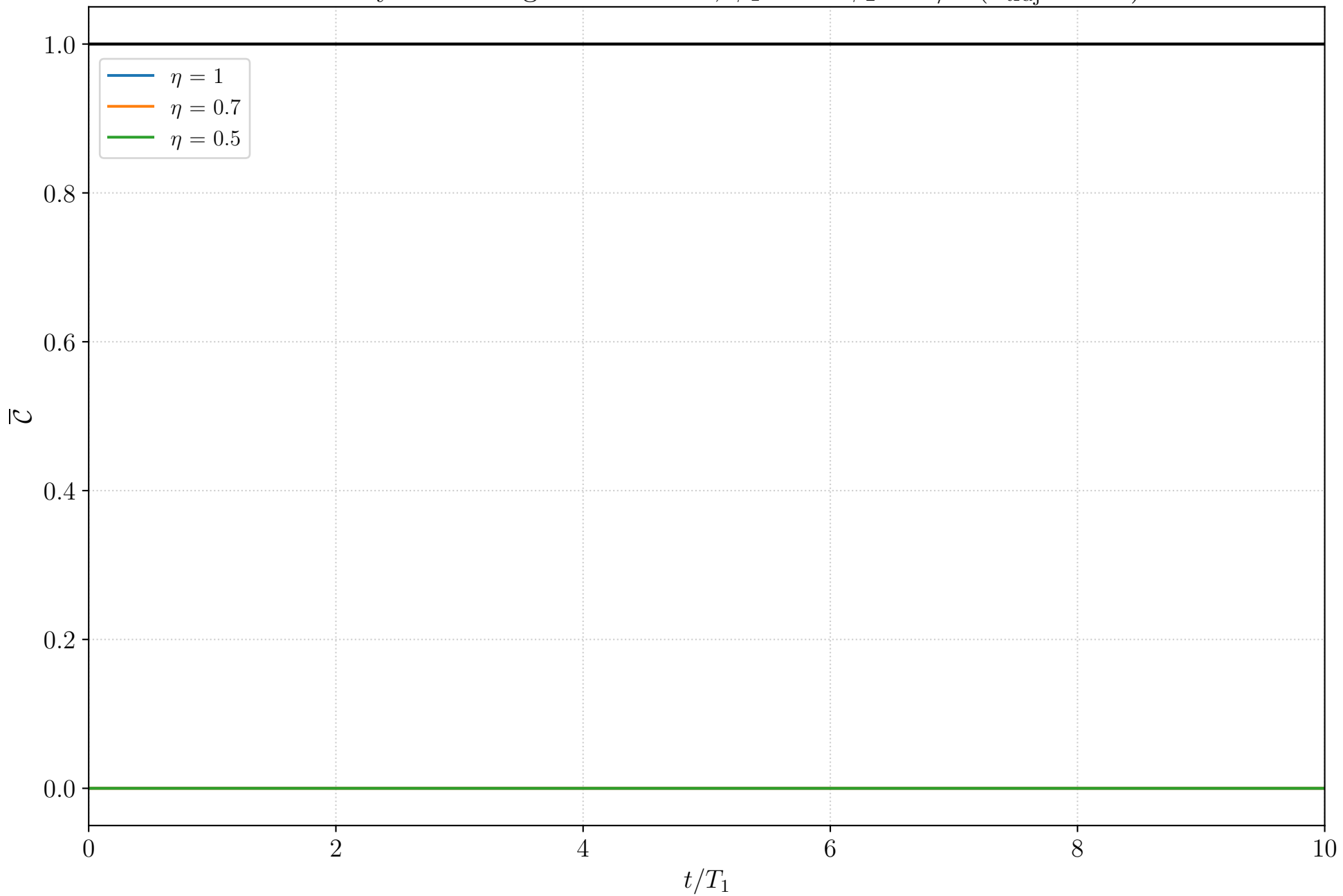
Heterodyne: Average \bar{\mathcal{C}} over time, \phi_1 = 0 \phi_2 = \pi/2 ( n_{\text{traj}} = 100 )
