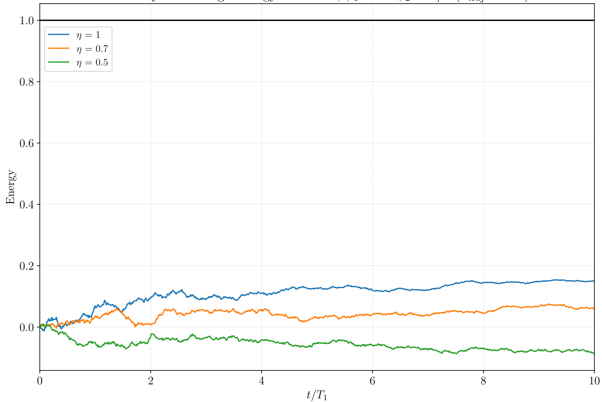
Heterodyne: Average Energy over time, \phi_1 = 0 \phi_2 = \pi/2 ( n_{\text{traj}} = 100 )
